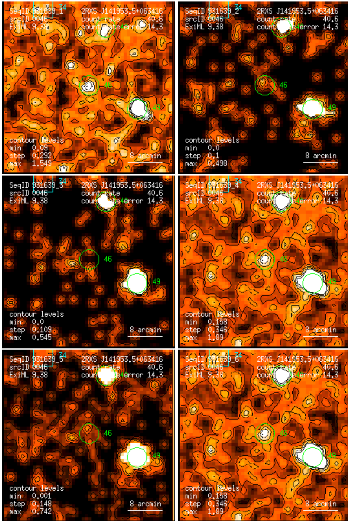
Figure 46: RASS 931639: detection 0046: band rate images, Gaussian filter: (1) PSPC channels 11 – 41, (2) 52 – 90, (3) 91 – 201, (4) 11 – 235, (5) 52 – 201, (6) 11 – 201. Broad band rates in counts/ks. Band rate contour levels in counts/ks/arcmin 2 .
