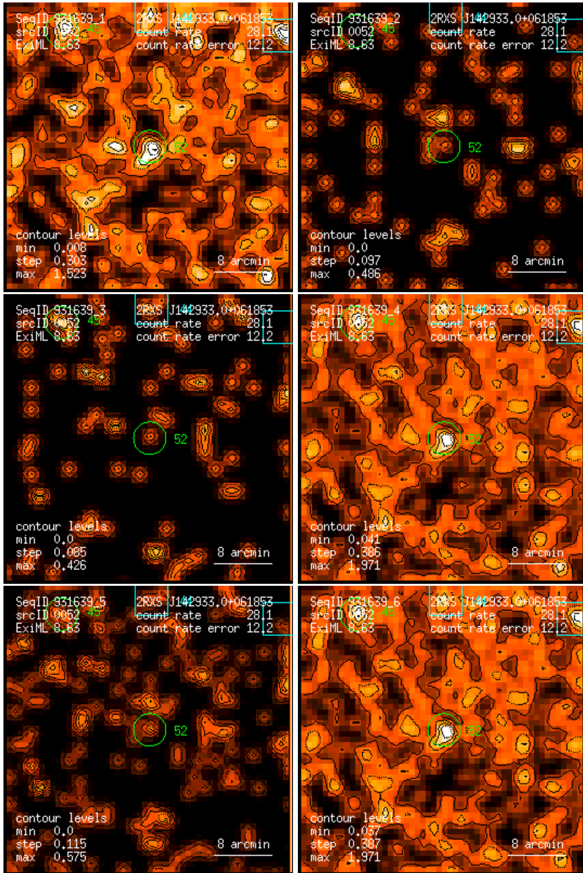
Figure 52: RASS 931639: detection 0052: band rate images, Gaussian filter: (1) PSPC channels 11 – 41, (2) 52 – 90, (3) 91 – 201, (4) 11 – 235, (5) 52 – 201, (6) 11 – 201. Broad band rates in counts/ks. Band rate contour levels in counts/ks/arcmin 2 .
