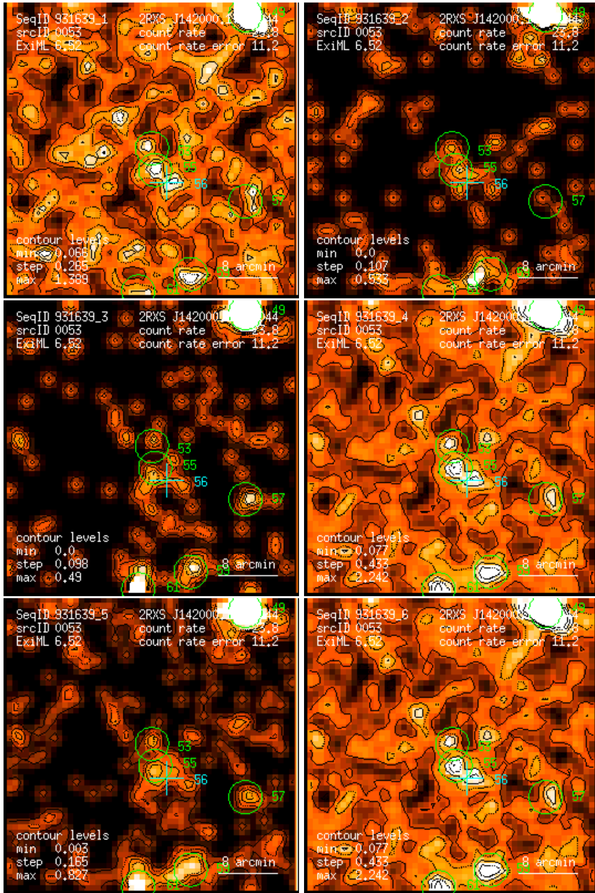
Figure 53: RASS 931639: detection 0053: band rate images, Gaussian filter: (1) PSPC channels 11 – 41, (2) 52 – 90, (3) 91 – 201, (4) 11 – 235, (5) 52 – 201, (6) 11 – 201. Broad band rates in counts/ks. Band rate contour levels in counts/ks/arcmin 2 .
