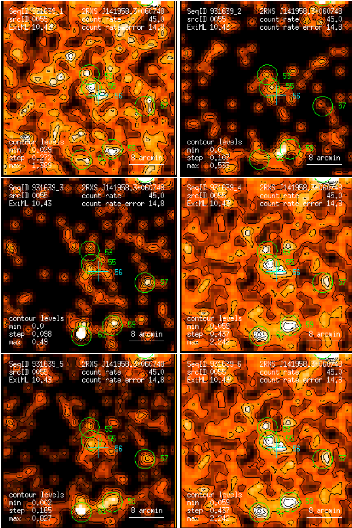
Figure 55: RASS 931639: detection 0055: band rate images, Gaussian filter: (1) PSPC channels 11 – 41, (2) 52 – 90, (3) 91 – 201, (4) 11 – 235, (5) 52 – 201, (6) 11 – 201. Broad band rates in counts/ks. Band rate contour levels in counts/ks/arcmin 2 .
