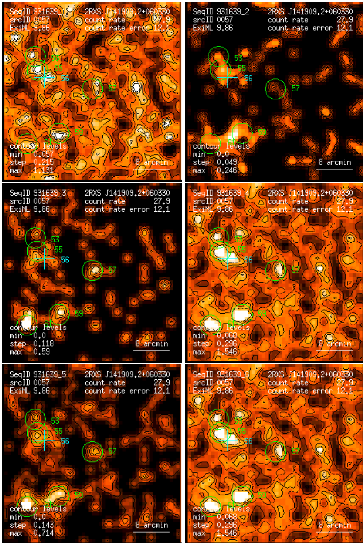
Figure 57: RASS 931639: detection 0057: band rate images, Gaussian filter: (1) PSPC channels 11 – 41, (2) 52 – 90, (3) 91 – 201, (4) 11 – 235, (5) 52 – 201, (6) 11 – 201. Broad band rates in counts/ks. Band rate contour levels in counts/ks/arcmin 2 .
