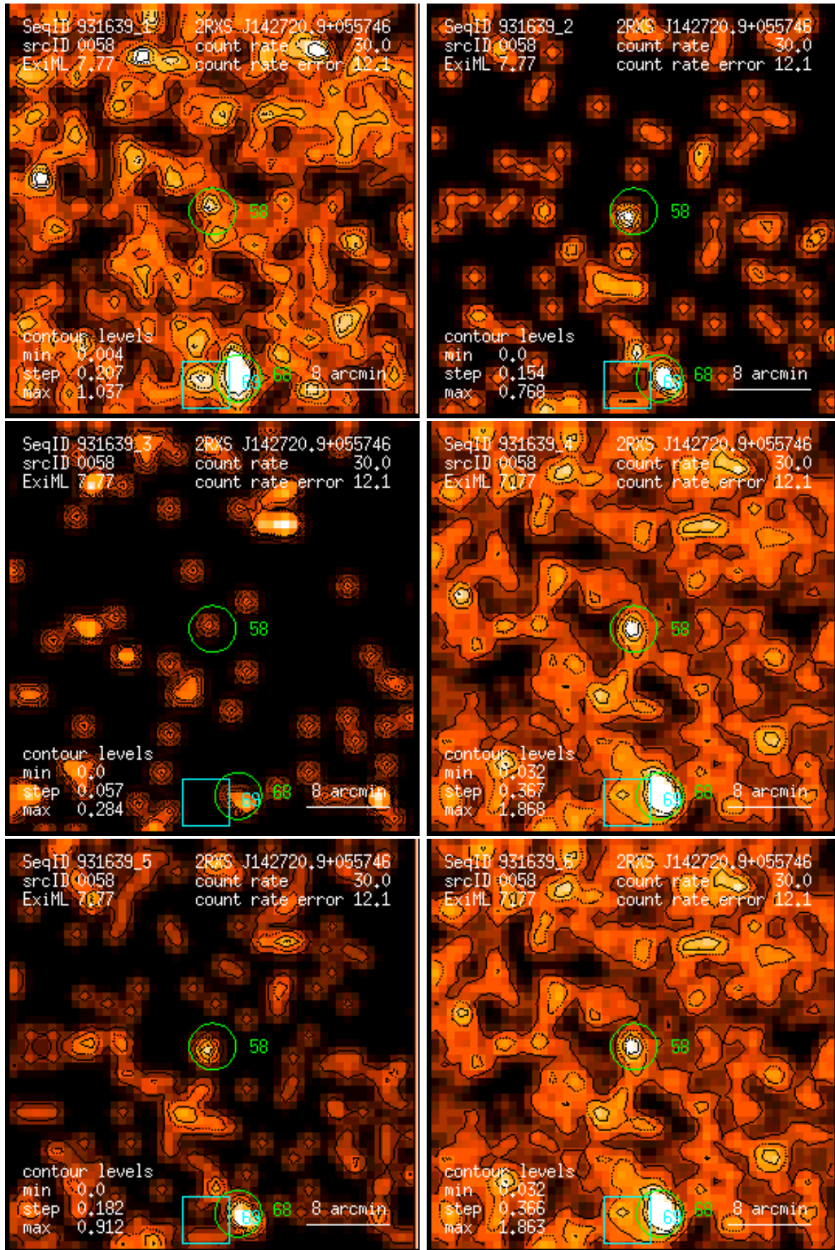
Figure 58: RASS 931639: detection 0058: band rate images, Gaussian filter: (1) PSPC channels 11 – 41, (2) 52 – 90, (3) 91 – 201, (4) 11 – 235, (5) 52 – 201, (6) 11 – 201. Broad band rates in counts/ks. Band rate contour levels in counts/ks/arcmin 2 .
