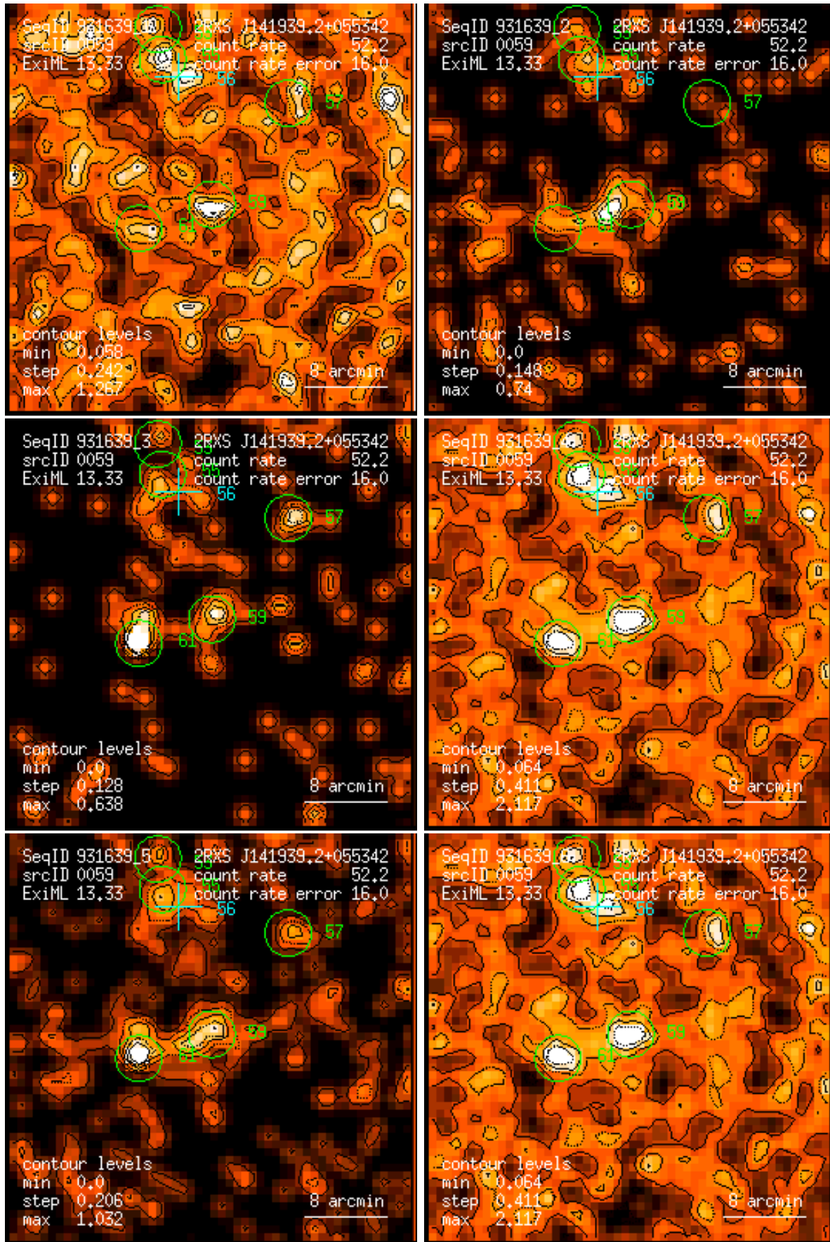
Figure 59: RASS 931639: detection 0059: band rate images, Gaussian filter: (1) PSPC channels 11 – 41, (2) 52 – 90, (3) 91 – 201, (4) 11 – 235, (5) 52 – 201, (6) 11 – 201. Broad band rates in counts/ks. Band rate contour levels in counts/ks/arcmin 2 .
