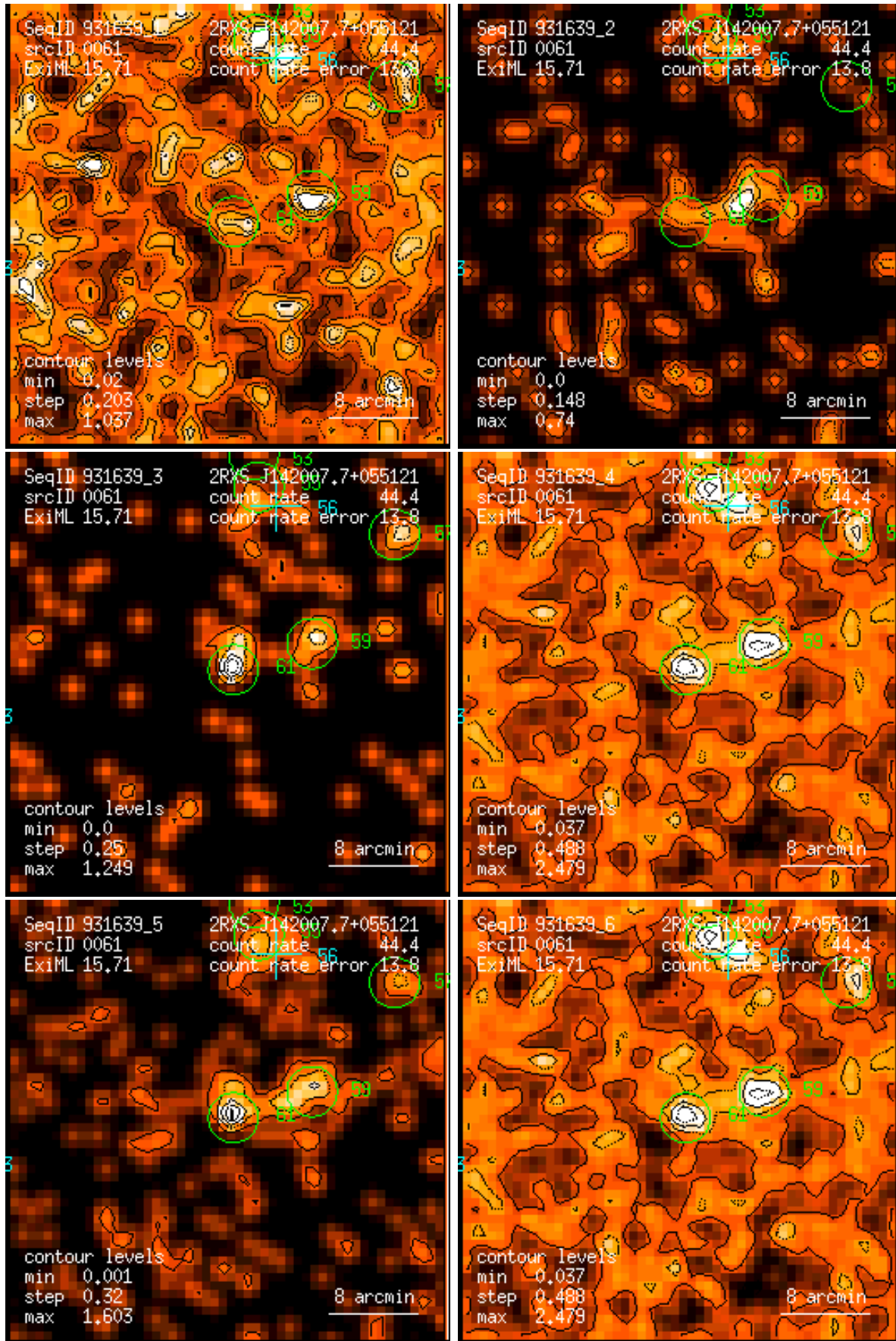
Figure 61: RASS 931639: detection 0061: band rate images, Gaussian filter: (1) PSPC channels 11 – 41, (2) 52 – 90, (3) 91 – 201, (4) 11 – 235, (5) 52 – 201, (6) 11 – 201. Broad band rates in counts/ks. Band rate contour levels in counts/ks/arcmin 2 .
