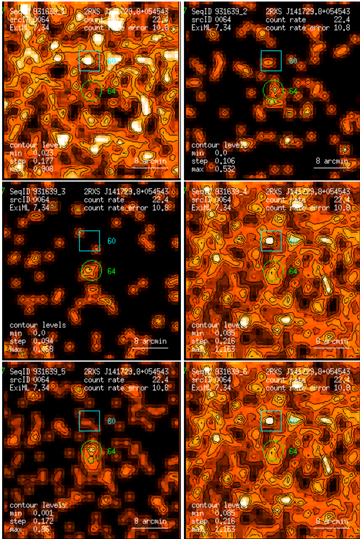
Figure 64: RASS 931639: detection 0064: band rate images, Gaussian filter: (1) PSPC channels 11 – 41, (2) 52 – 90, (3) 91 – 201, (4) 11 – 235, (5) 52 – 201, (6) 11 – 201. Broad band rates in counts/ks. Band rate contour levels in counts/ks/arcmin 2 .
