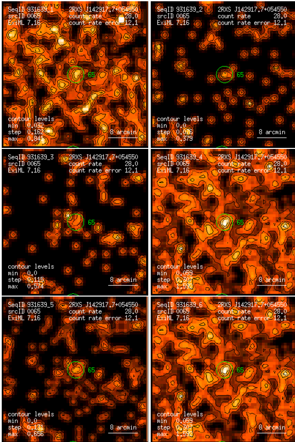
Figure 65: RASS 931639: detection 0065: band rate images, Gaussian filter: (1) PSPC channels 11 – 41, (2) 52 – 90, (3) 91 – 201, (4) 11 – 235, (5) 52 – 201, (6) 11 – 201. Broad band rates in counts/ks. Band rate contour levels in counts/ks/arcmin 2 .
