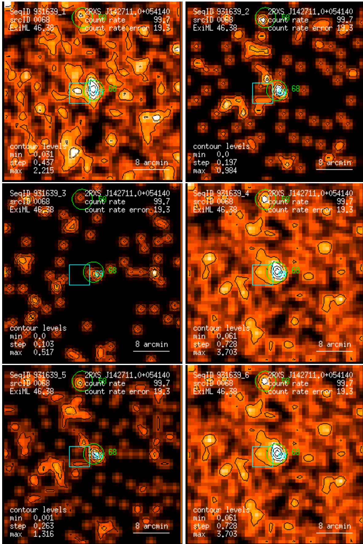
Figure 68: RASS 931639: detection 0068: band rate images, Gaussian filter: (1) PSPC channels 11 – 41, (2) 52 – 90, (3) 91 – 201, (4) 11 – 235, (5) 52 – 201, (6) 11 – 201. Broad band rates in counts/ks. Band rate contour levels in counts/ks/arcmin 2 .
