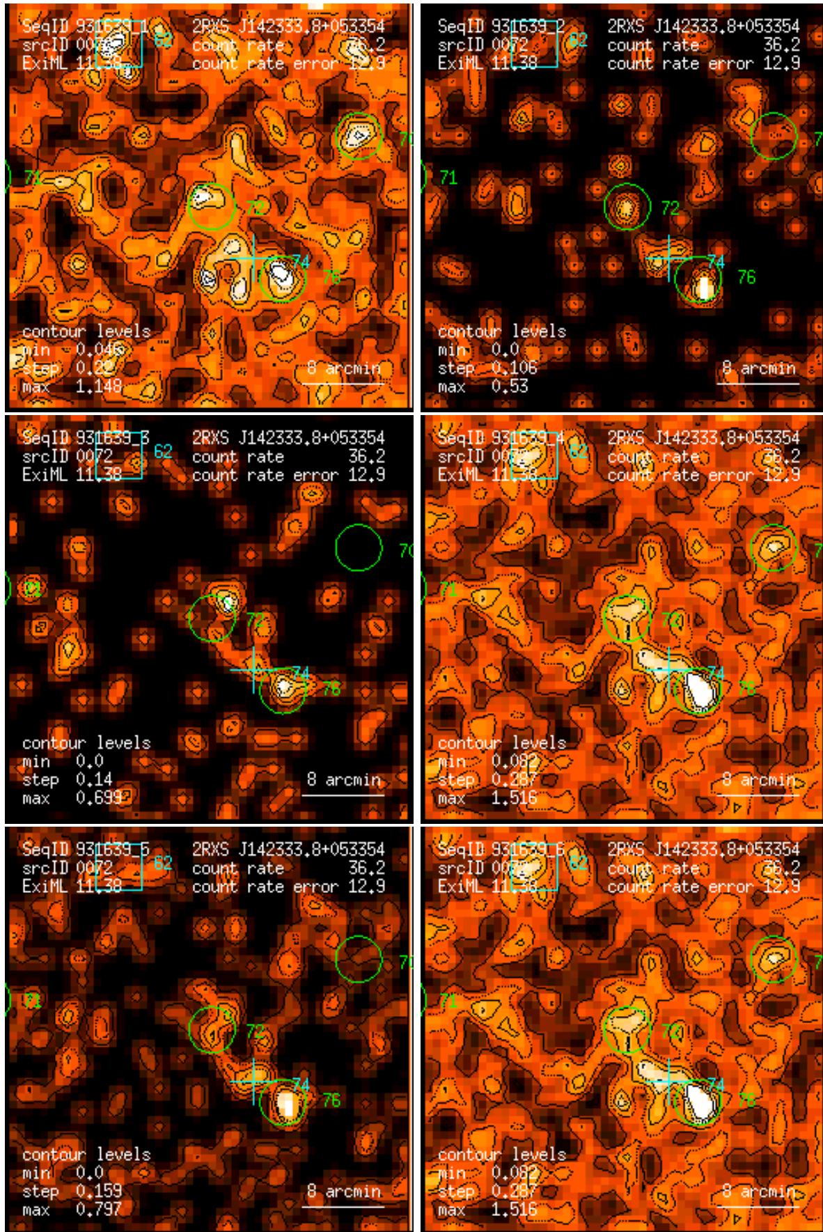
Figure 72: RASS 931639: detection 0072: band rate images, Gaussian filter: (1) PSPC channels 11 – 41, (2) 52 – 90, (3) 91 – 201, (4) 11 – 235, (5) 52 – 201, (6) 11 – 201. Broad band rates in counts/ks. Band rate contour levels in counts/ks/arcmin 2 .
