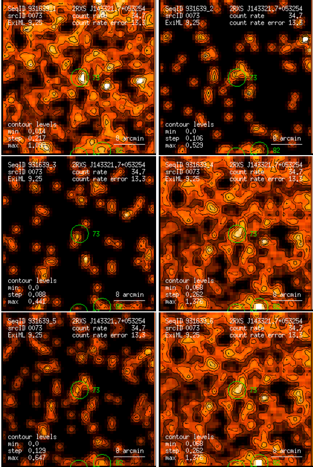
Figure 73: RASS 931639: detection 0073: band rate images, Gaussian filter: (1) PSPC channels 11 – 41, (2) 52 – 90, (3) 91 – 201, (4) 11 – 235, (5) 52 – 201, (6) 11 – 201. Broad band rates in counts/ks. Band rate contour levels in counts/ks/arcmin 2 .
