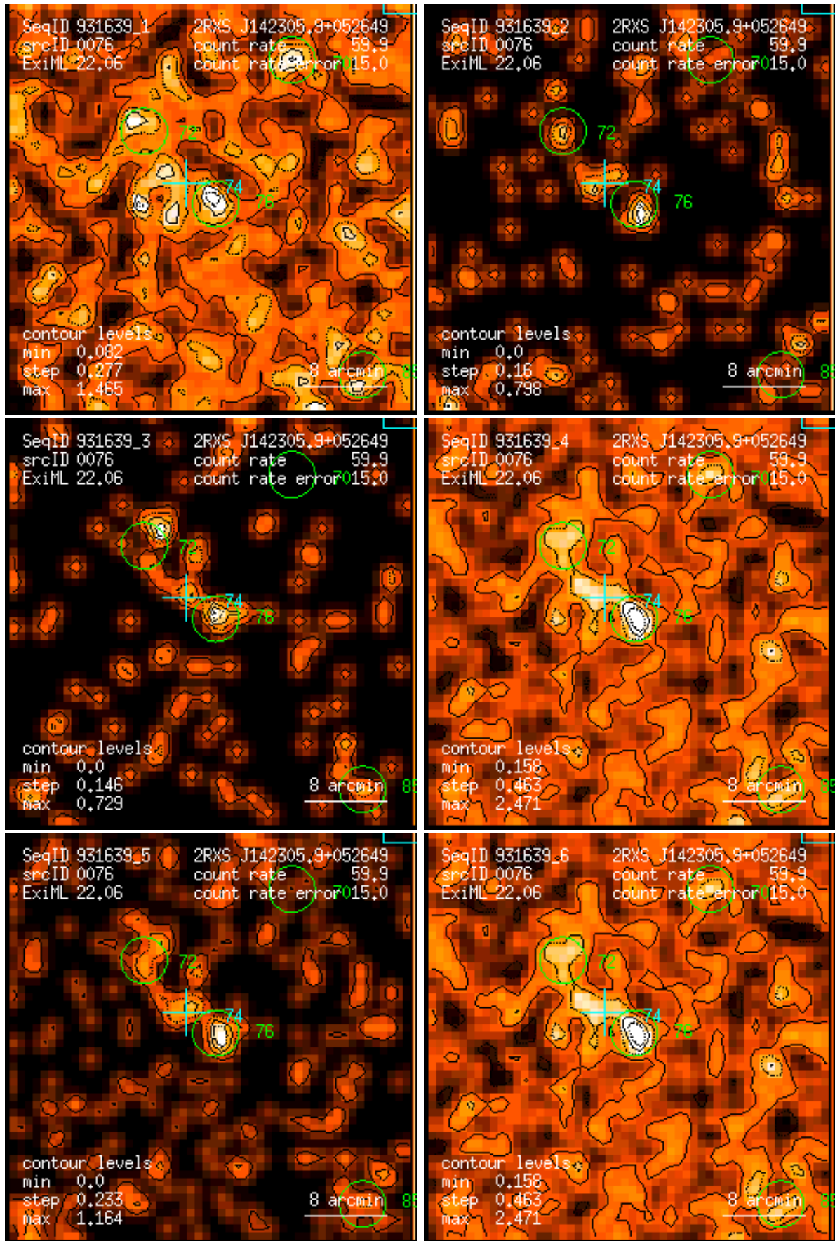
Figure 76: RASS 931639: detection 0076: band rate images, Gaussian filter: (1) PSPC channels 11 – 41, (2) 52 – 90, (3) 91 – 201, (4) 11 – 235, (5) 52 – 201, (6) 11 – 201. Broad band rates in counts/ks. Band rate contour levels in counts/ks/arcmin 2 .
