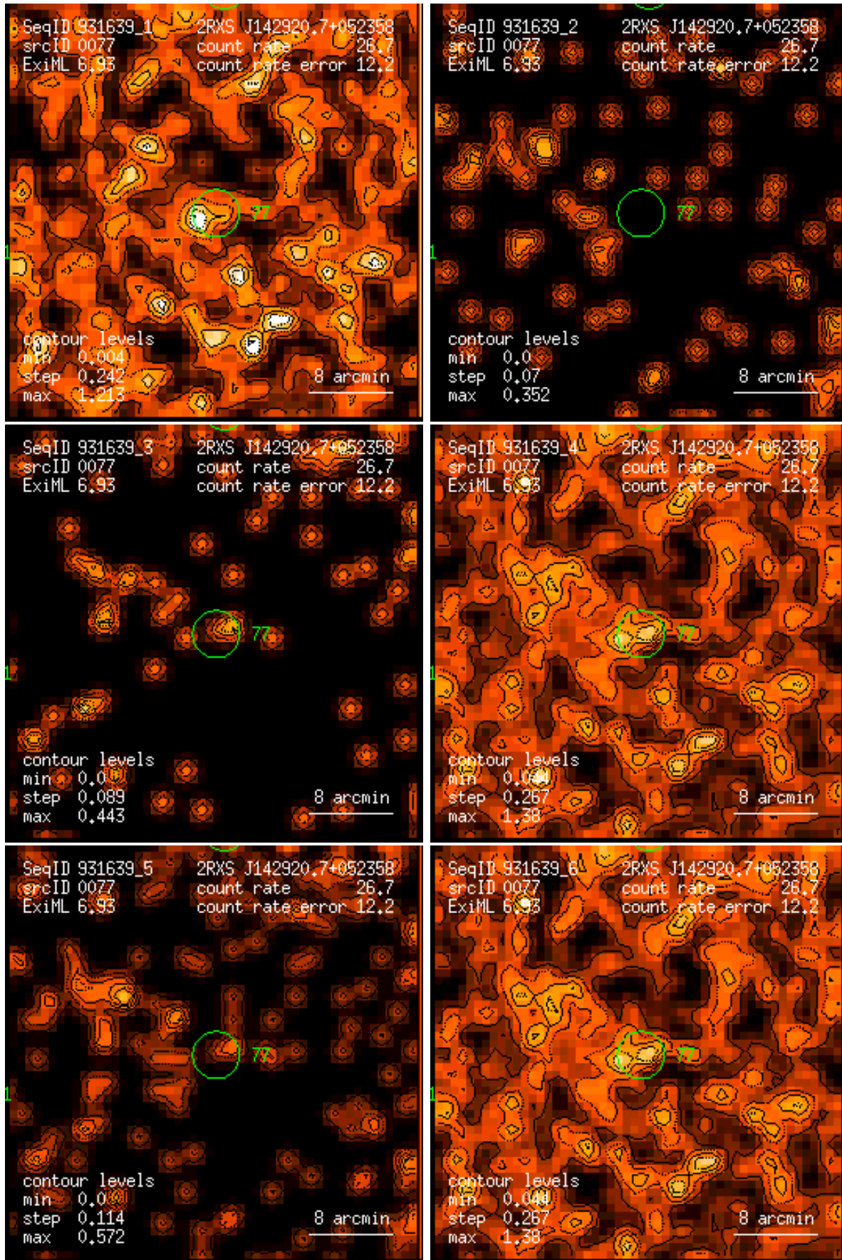
Figure 77: RASS 931639: detection 0077: band rate images, Gaussian filter: (1) PSPC channels 11 – 41, (2) 52 – 90, (3) 91 – 201, (4) 11 – 235, (5) 52 – 201, (6) 11 – 201. Broad band rates in counts/ks. Band rate contour levels in counts/ks/arcmin 2 .
