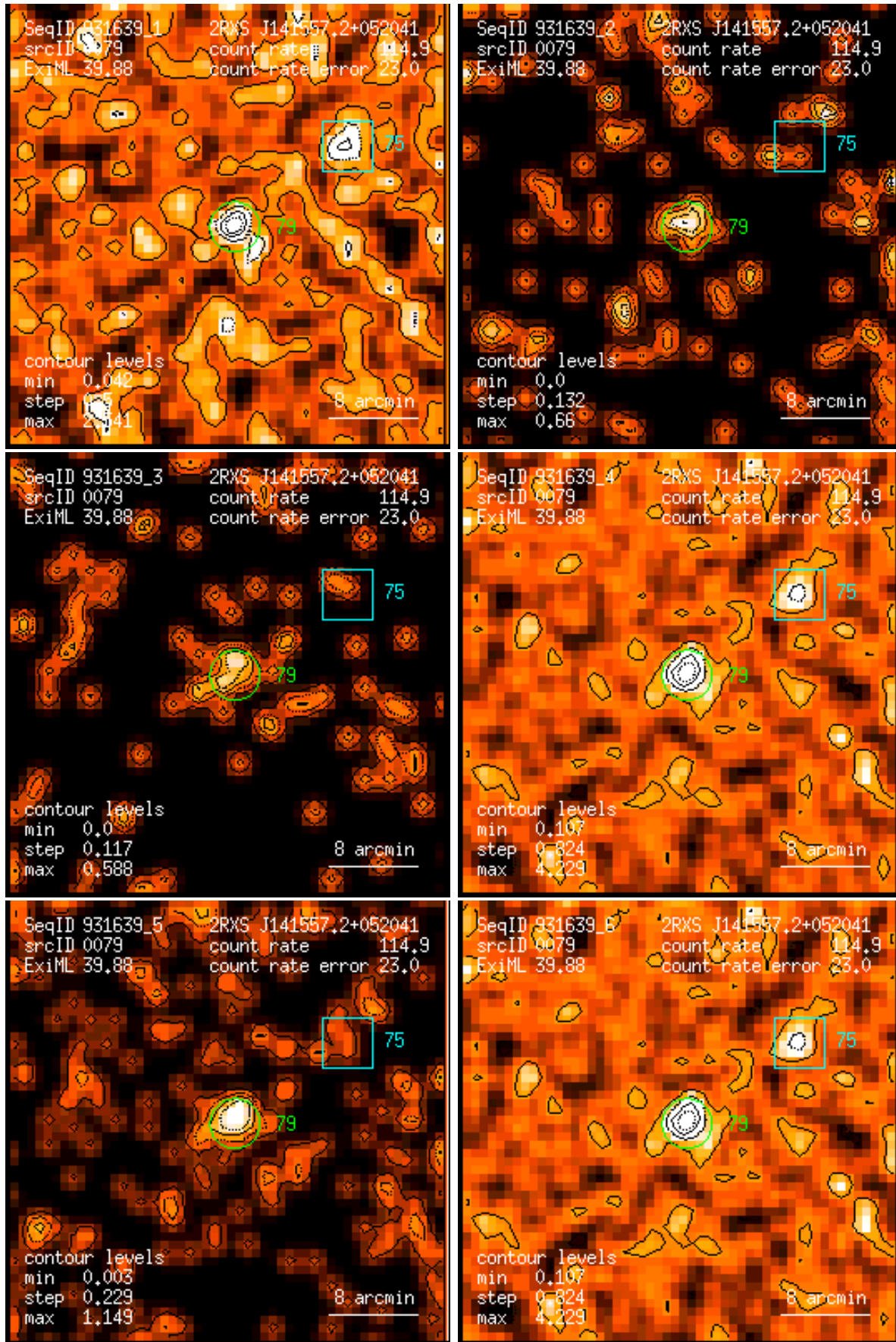
Figure 79: RASS 931639: detection 0079: band rate images, Gaussian filter: (1) PSPC channels 11 – 41, (2) 52 – 90, (3) 91 – 201, (4) 11 – 235, (5) 52 – 201, (6) 11 – 201. Broad band rates in counts/ks. Band rate contour levels in counts/ks/arcmin 2 .
