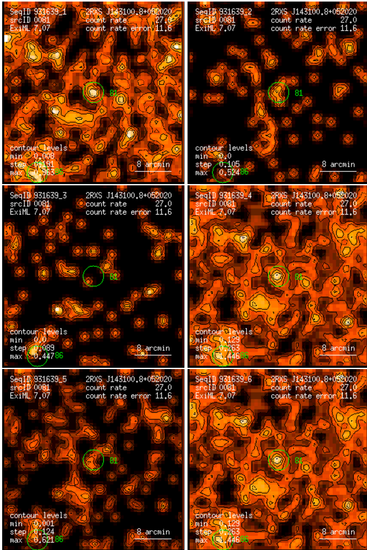
Figure 81: RASS 931639: detection 0081: band rate images, Gaussian filter: (1) PSPC channels 11 – 41, (2) 52 – 90, (3) 91 – 201, (4) 11 – 235, (5) 52 – 201, (6) 11 – 201. Broad band rates in counts/ks. Band rate contour levels in counts/ks/arcmin 2 .
