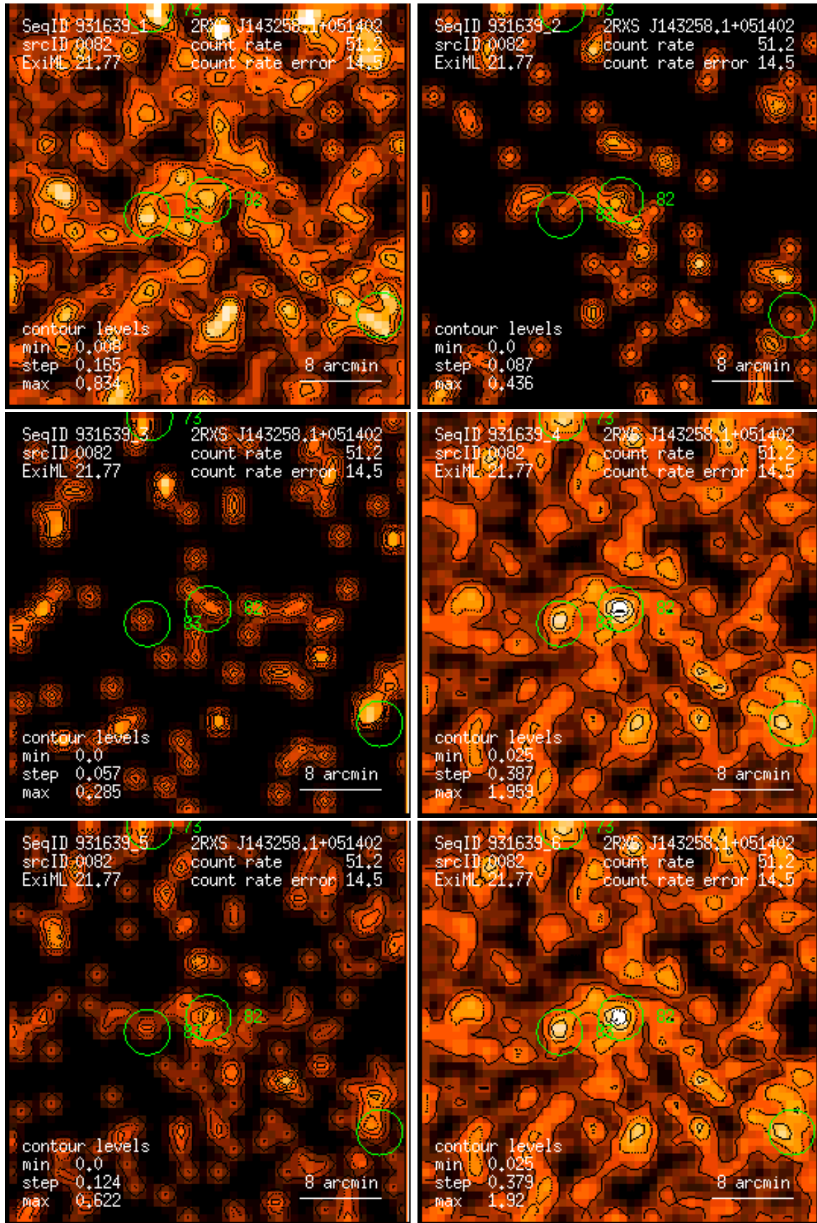
Figure 82: RASS 931639: detection 0082: band rate images, Gaussian filter: (1) PSPC channels 11 – 41, (2) 52 – 90, (3) 91 – 201, (4) 11 – 235, (5) 52 – 201, (6) 11 – 201. Broad band rates in counts/ks. Band rate contour levels in counts/ks/arcmin 2 .
