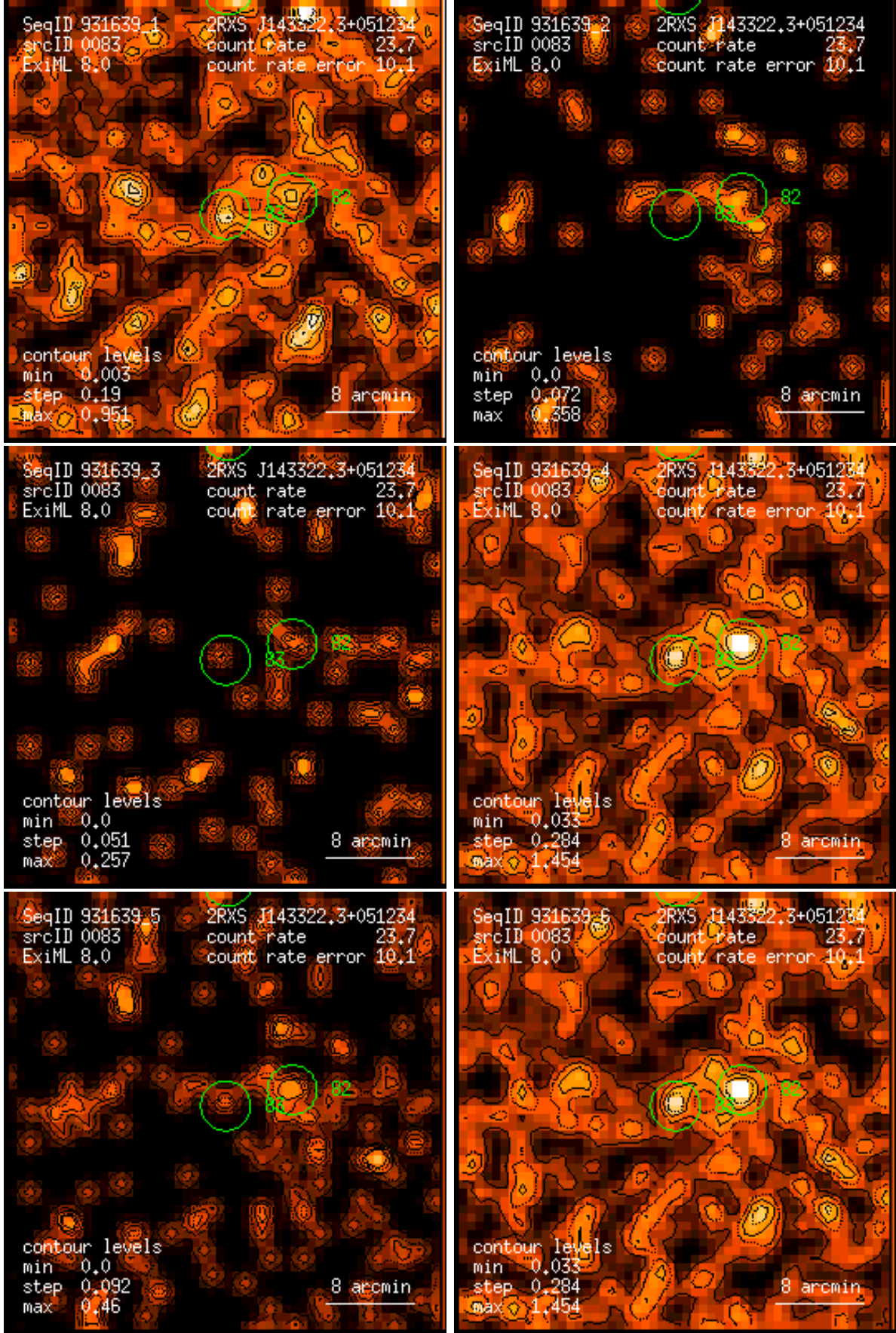
Figure 83: RASS 931639: detection 0083: band rate images, Gaussian filter: (1) PSPC channels 11 – 41, (2) 52 – 90, (3) 91 – 201, (4) 11 – 235, (5) 52 – 201, (6) 11 – 201. Broad band rates in counts/ks. Band rate contour levels in counts/ks/arcmin 2 .
