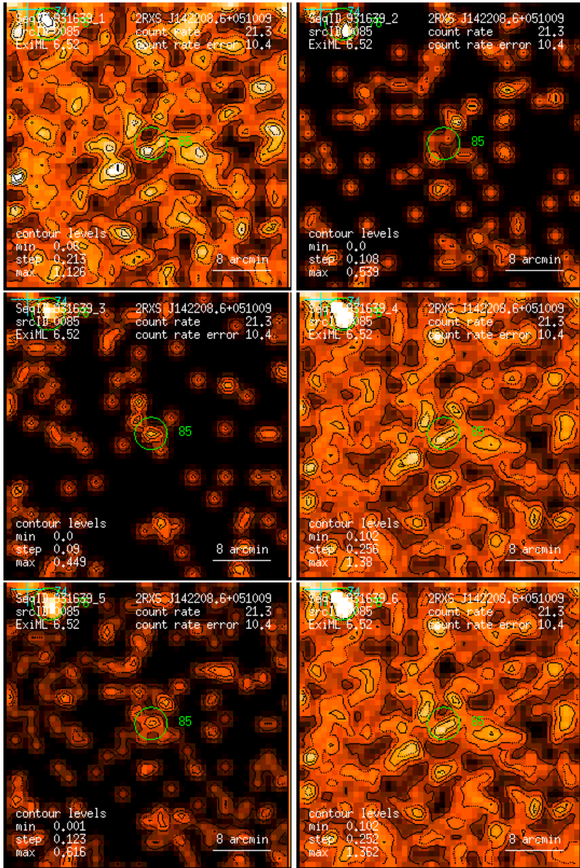
Figure 85: RASS 931639: detection 0085: band rate images, Gaussian filter: (1) PSPC channels 11 – 41, (2) 52 – 90, (3) 91 – 201, (4) 11 – 235, (5) 52 – 201, (6) 11 – 201. Broad band rates in counts/ks. Band rate contour levels in counts/ks/arcmin 2 .
