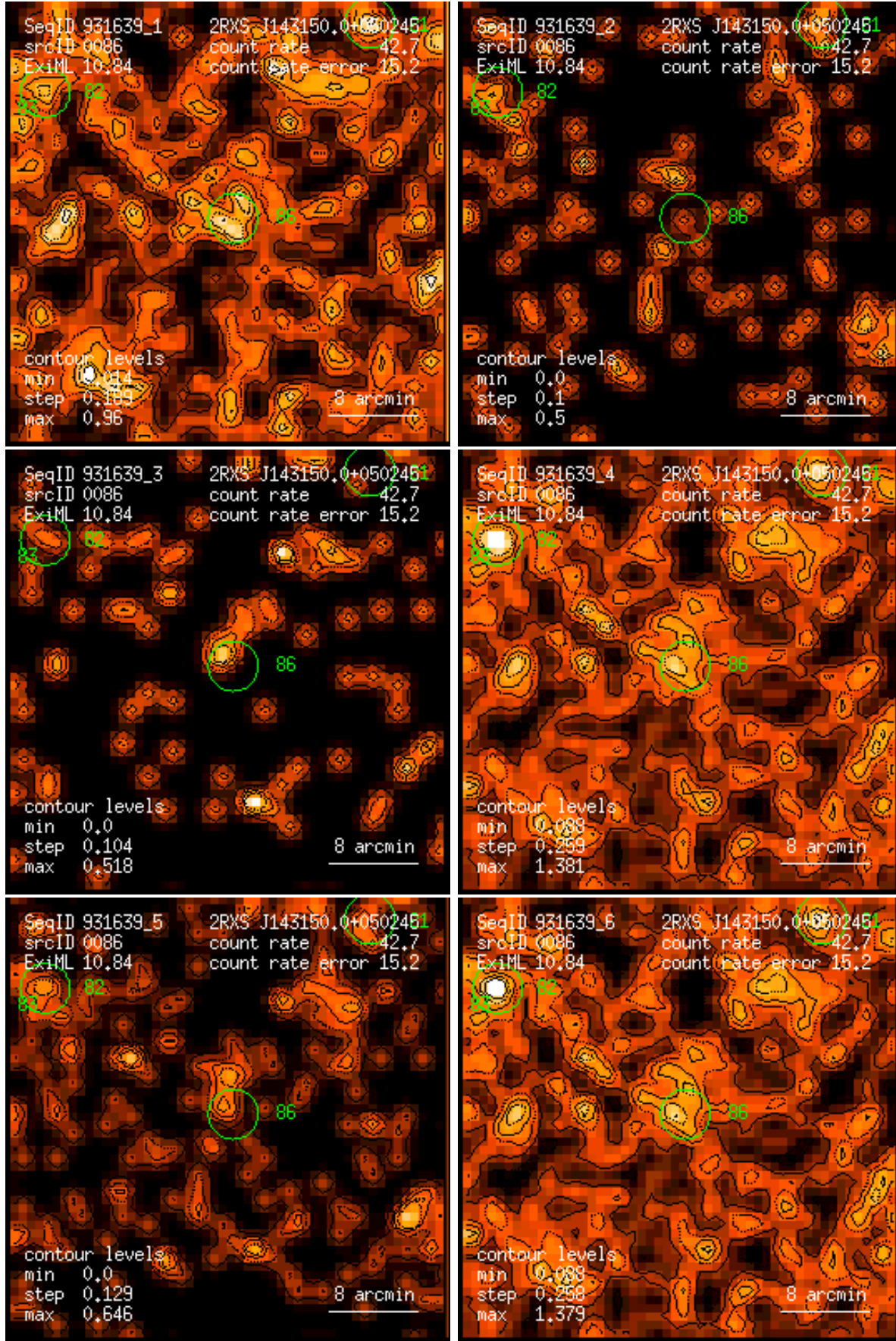
Figure 86: RASS 931639: detection 0086: band rate images, Gaussian filter: (1) PSPC channels 11 – 41, (2) 52 – 90, (3) 91 – 201, (4) 11 – 235, (5) 52 – 201, (6) 11 – 201. Broad band rates in counts/ks. Band rate contour levels in counts/ks/arcmin 2 .
