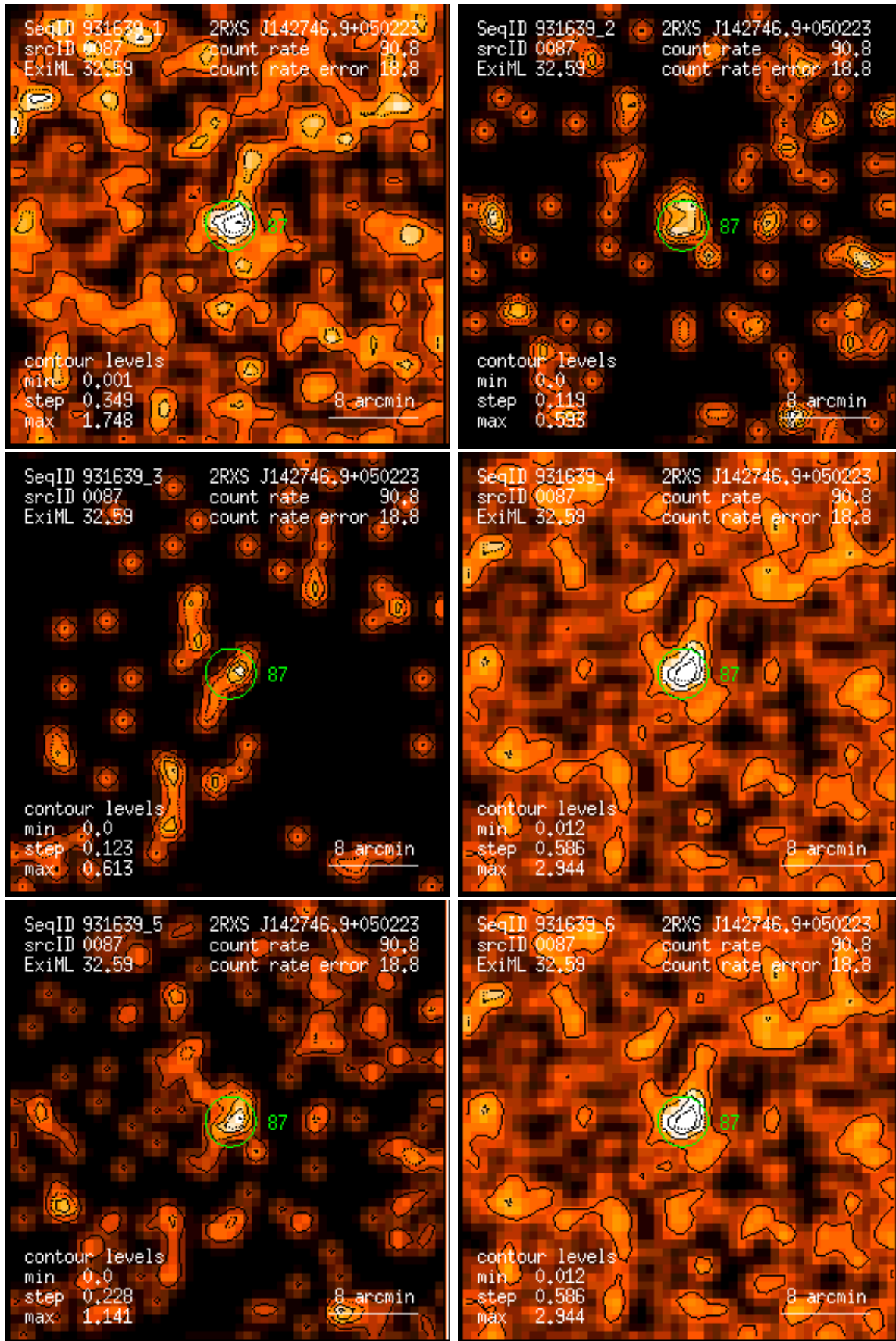
Figure 87: RASS 931639: detection 0087: band rate images, Gaussian filter: (1) PSPC channels 11 – 41, (2) 52 – 90, (3) 91 – 201, (4) 11 – 235, (5) 52 – 201, (6) 11 – 201. Broad band rates in counts/ks. Band rate contour levels in counts/ks/arcmin 2 .
