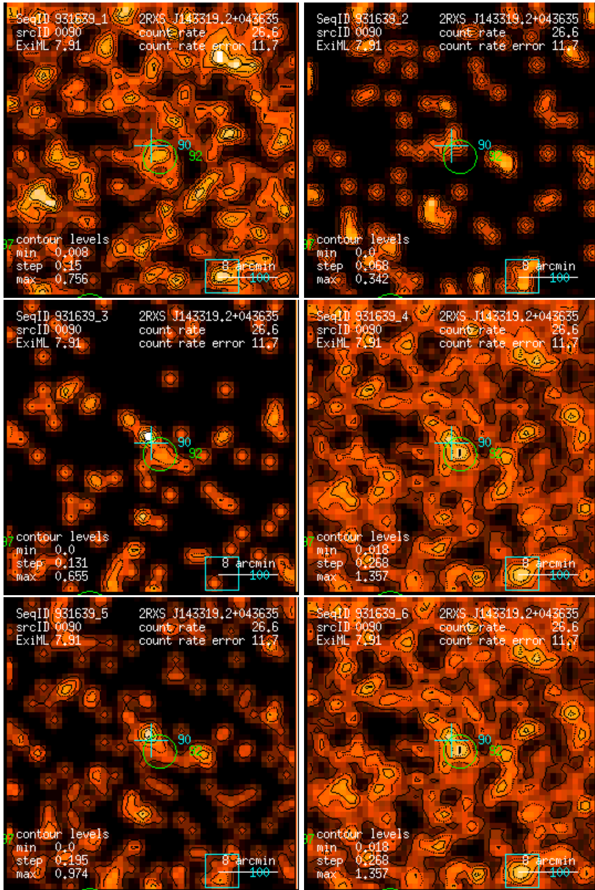
Figure 90: RASS 931639: detection 0090: band rate images, Gaussian filter: (1) PSPC channels 11 – 41, (2) 52 – 90, (3) 91 – 201, (4) 11 – 235, (5) 52 – 201, (6) 11 – 201. Broad band rates in counts/ks. Band rate contour levels in counts/ks/arcmin 2 .
