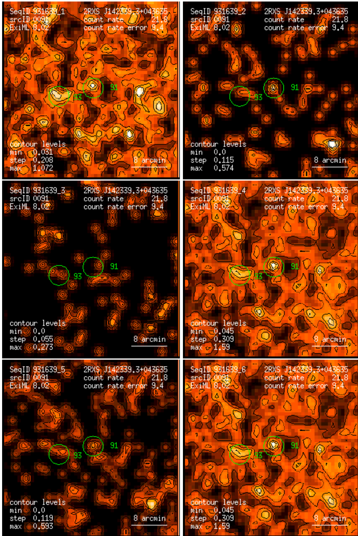
Figure 91: RASS 931639: detection 0091: band rate images, Gaussian filter: (1) PSPC channels 11 – 41, (2) 52 – 90, (3) 91 – 201, (4) 11 – 235, (5) 52 – 201, (6) 11 – 201. Broad band rates in counts/ks. Band rate contour levels in counts/ks/arcmin 2 .
