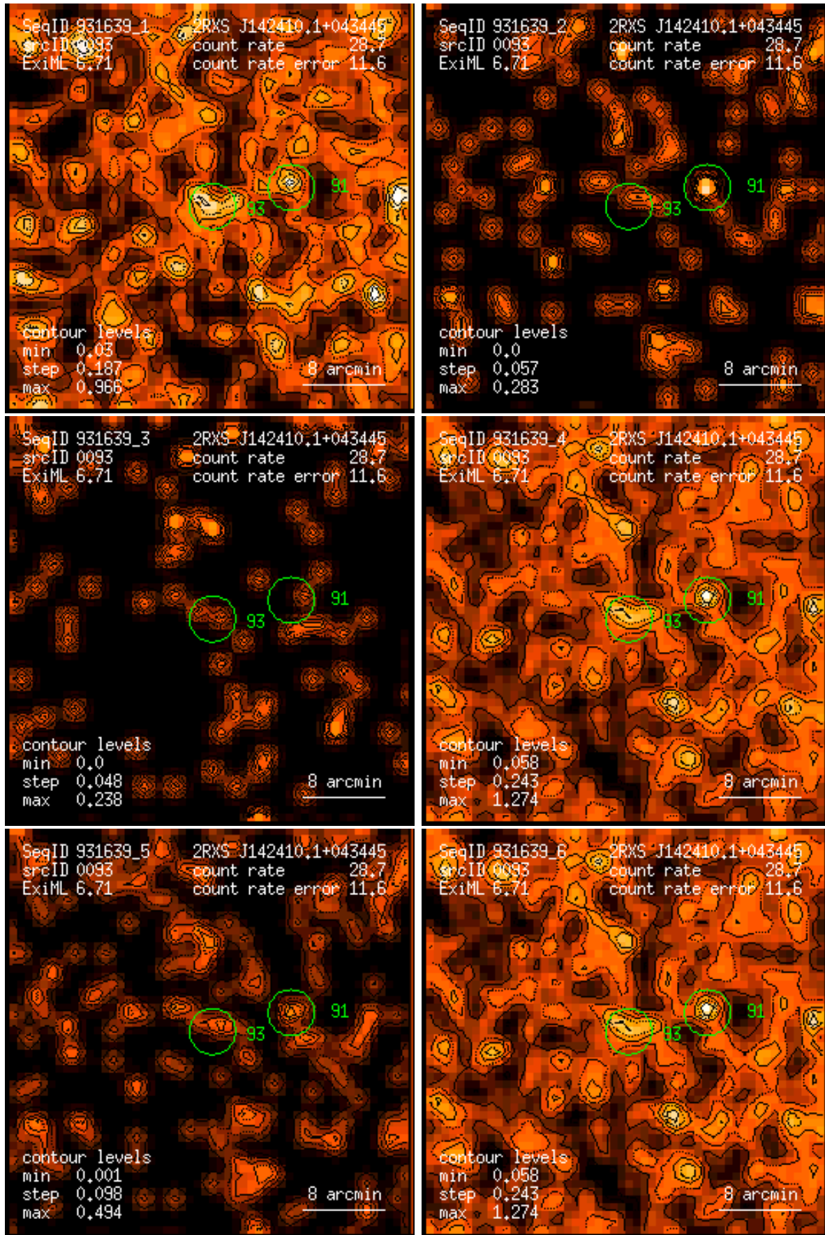
Figure 93: RASS 931639: detection 0093: band rate images, Gaussian filter: (1) PSPC channels 11 – 41, (2) 52 – 90, (3) 91 – 201, (4) 11 – 235, (5) 52 – 201, (6) 11 – 201. Broad band rates in counts/ks. Band rate contour levels in counts/ks/arcmin 2 .
