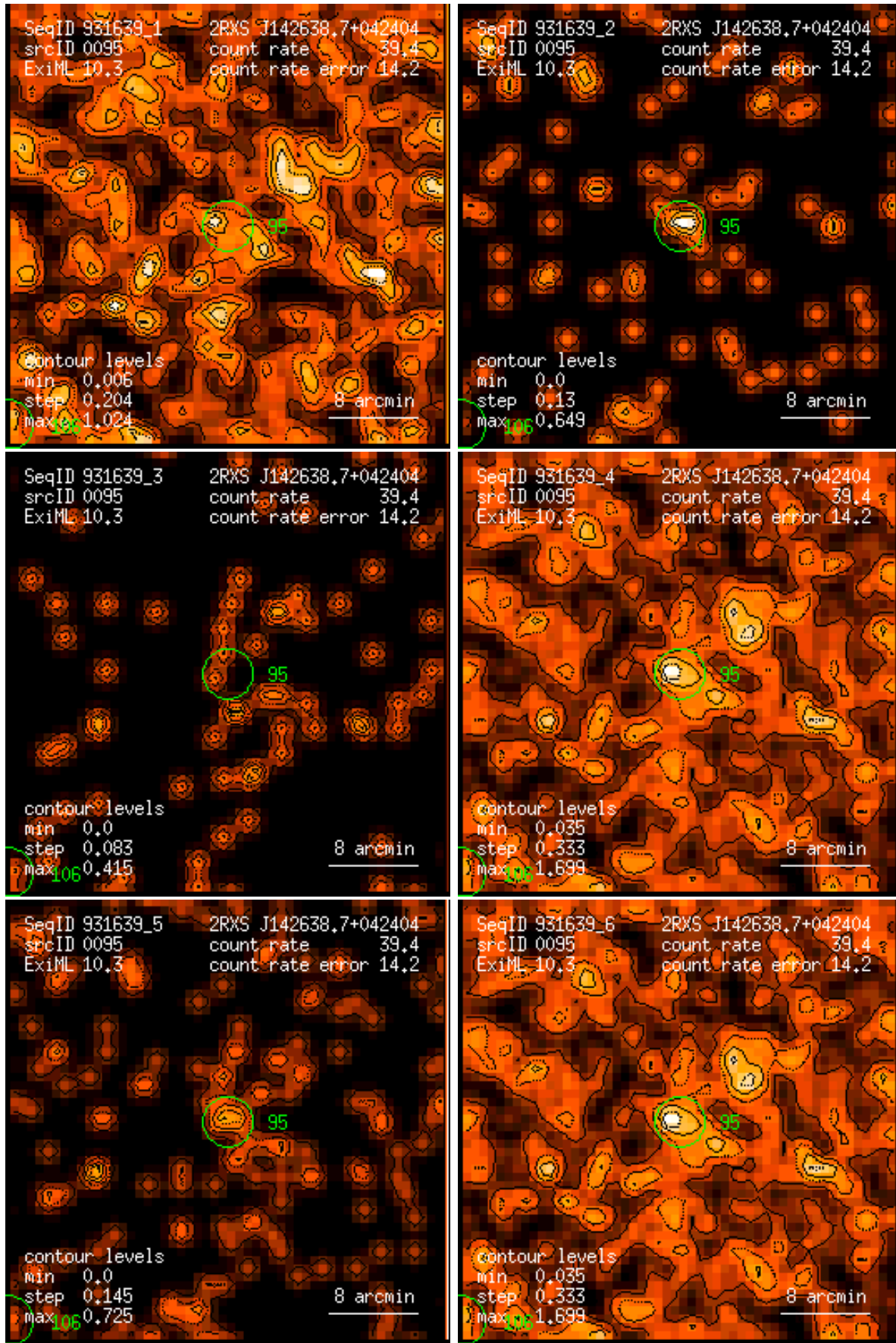
Figure 95: RASS 931639: detection 0095: band rate images, Gaussian filter: (1) PSPC channels 11 – 41, (2) 52 – 90, (3) 91 – 201, (4) 11 – 235, (5) 52 – 201, (6) 11 – 201. Broad band rates in counts/ks. Band rate contour levels in counts/ks/arcmin 2 .
