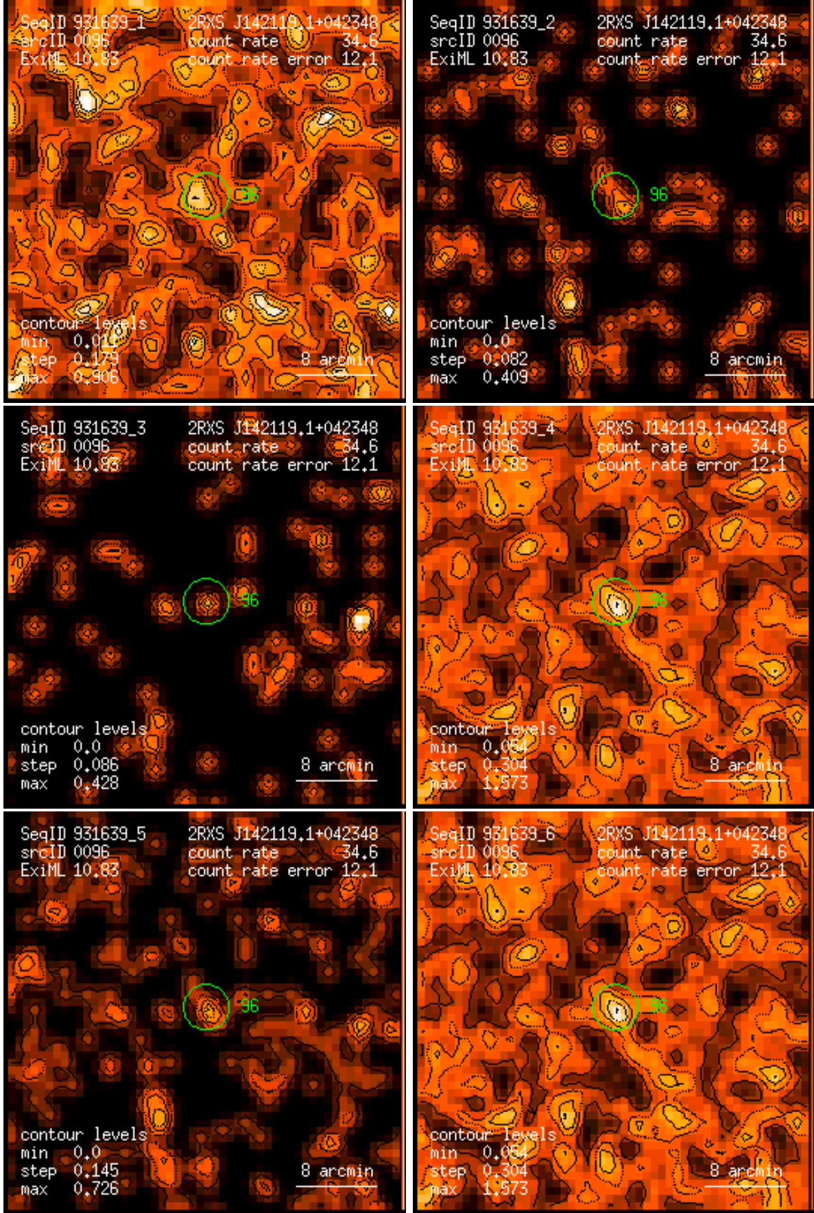
Figure 96: RASS 931639: detection 0096: band rate images, Gaussian filter: (1) PSPC channels 11 – 41, (2) 52 – 90, (3) 91 – 201, (4) 11 – 235, (5) 52 – 201, (6) 11 – 201. Broad band rates in counts/ks. Band rate contour levels in counts/ks/arcmin 2 .
