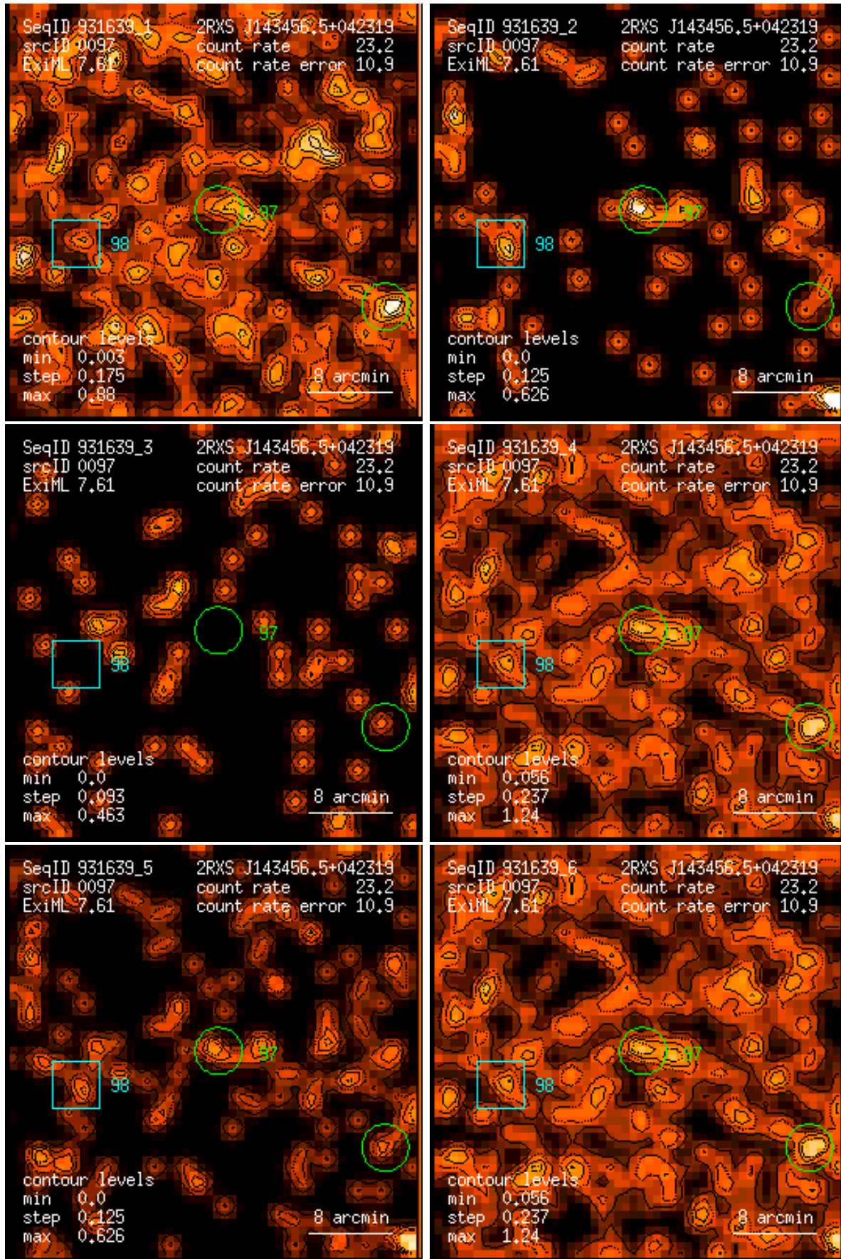
Figure 97: RASS 931639: detection 0097: band rate images, Gaussian filter: (1) PSPC channels 11 – 41, (2) 52 – 90, (3) 91 – 201, (4) 11 – 235, (5) 52 – 201, (6) 11 – 201. Broad band rates in counts/ks. Band rate contour levels in counts/ks/arcmin 2 .
