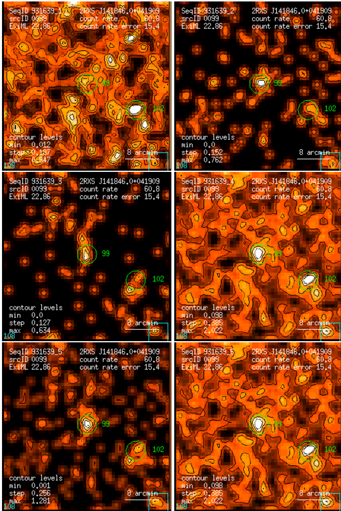
Figure 99: RASS 931639: detection 0099: band rate images, Gaussian filter: (1) PSPC channels 11 – 41, (2) 52 – 90, (3) 91 – 201, (4) 11 – 235, (5) 52 – 201, (6) 11 – 201. Broad band rates in counts/ks. Band rate contour levels in counts/ks/arcmin 2 .
