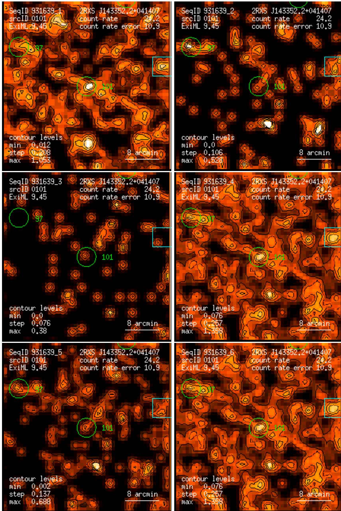
Figure 101: RASS 931639: detection 0101: band rate images, Gaussian filter: (1) PSPC channels 11 – 41, (2) 52 – 90, (3) 91 – 201, (4) 11 – 235, (5) 52 – 201, (6) 11 – 201. Broad band rates in counts/ks. Band rate contour levels in counts/ks/arcmin 2 .
