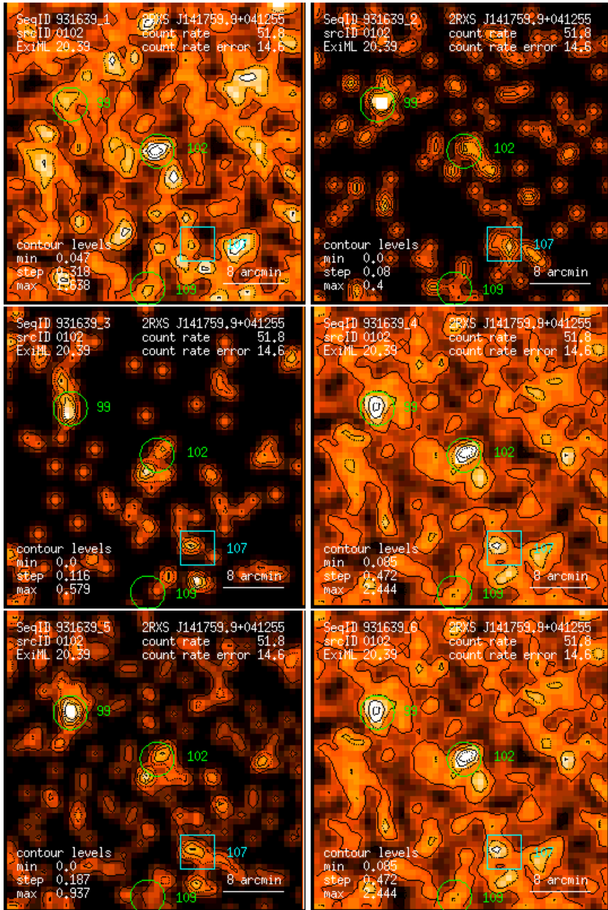
Figure 102: RASS 931639: detection 0102: band rate images, Gaussian filter: (1) PSPC channels 11 – 41, (2) 52 – 90, (3) 91 – 201, (4) 11 – 235, (5) 52 – 201, (6) 11 – 201. Broad band rates in counts/ks. Band rate contour levels in counts/ks/arcmin 2 .
