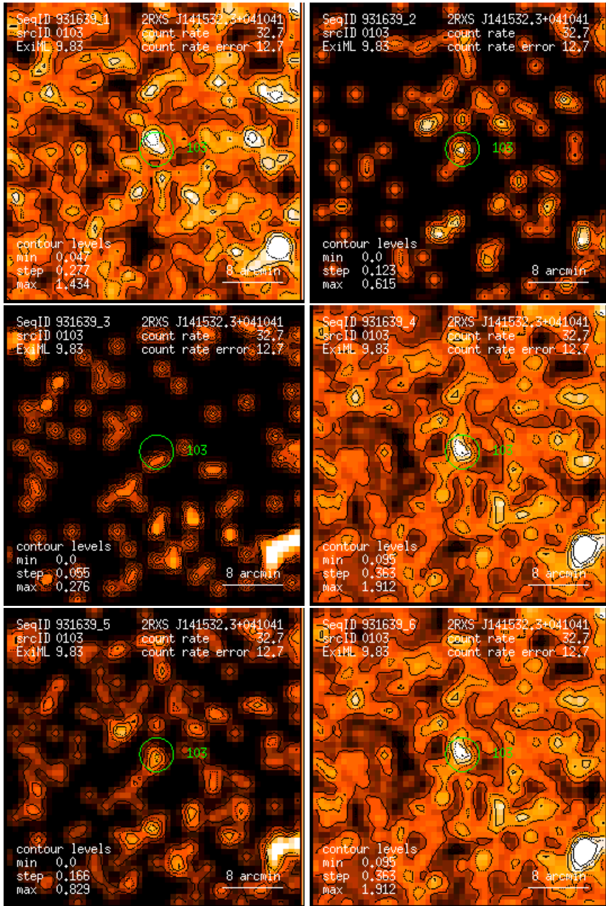
Figure 103: RASS 931639: detection 0103: band rate images, Gaussian filter: (1) PSPC channels 11 – 41, (2) 52 – 90, (3) 91 – 201, (4) 11 – 235, (5) 52 – 201, (6) 11 – 201. Broad band rates in counts/ks. Band rate contour levels in counts/ks/arcmin 2 .
