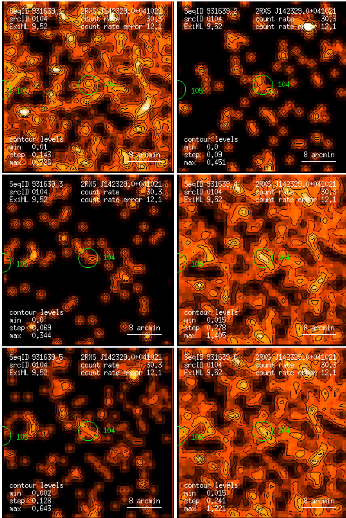
Figure 104: RASS 931639: detection 0104: band rate images, Gaussian filter: (1) PSPC channels 11 – 41, (2) 52 – 90, (3) 91 – 201, (4) 11 – 235, (5) 52 – 201, (6) 11 – 201. Broad band rates in counts/ks. Band rate contour levels in counts/ks/arcmin 2 .
