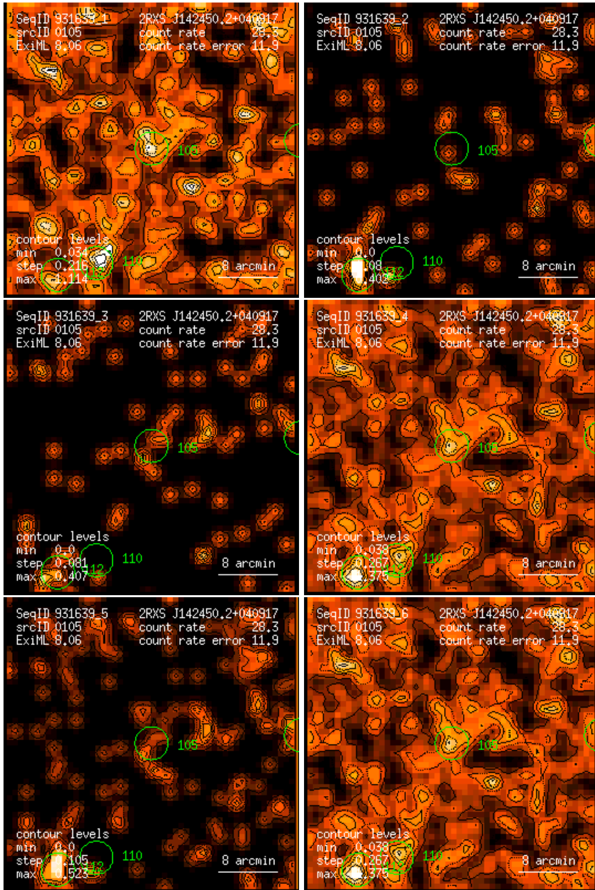
Figure 105: RASS 931639: detection 0105: band rate images, Gaussian filter: (1) PSPC channels 11 – 41, (2) 52 – 90, (3) 91 – 201, (4) 11 – 235, (5) 52 – 201, (6) 11 – 201. Broad band rates in counts/ks. Band rate contour levels in counts/ks/arcmin 2 .
