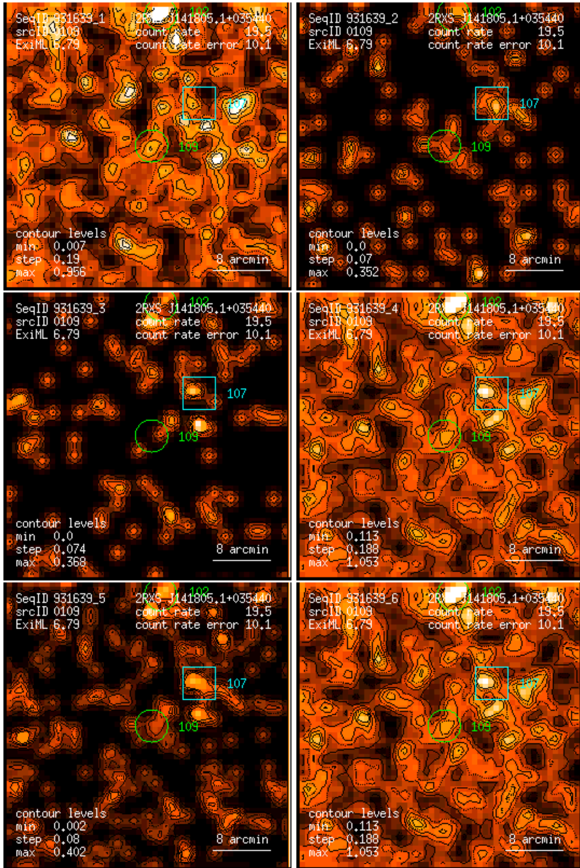
Figure 109: RASS 931639: detection 0109: band rate images, Gaussian filter: (1) PSPC channels 11 – 41, (2) 52 – 90, (3) 91 – 201, (4) 11 – 235, (5) 52 – 201, (6) 11 – 201. Broad band rates in counts/ks. Band rate contour levels in counts/ks/arcmin 2 .
