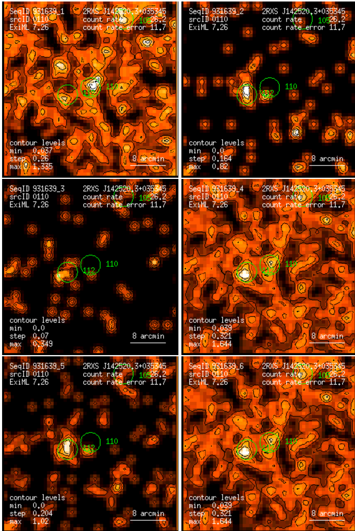
Figure 110: RASS 931639: detection 0110: band rate images, Gaussian filter: (1) PSPC channels 11 – 41, (2) 52 – 90, (3) 91 – 201, (4) 11 – 235, (5) 52 – 201, (6) 11 – 201. Broad band rates in counts/ks. Band rate contour levels in counts/ks/arcmin 2 .
