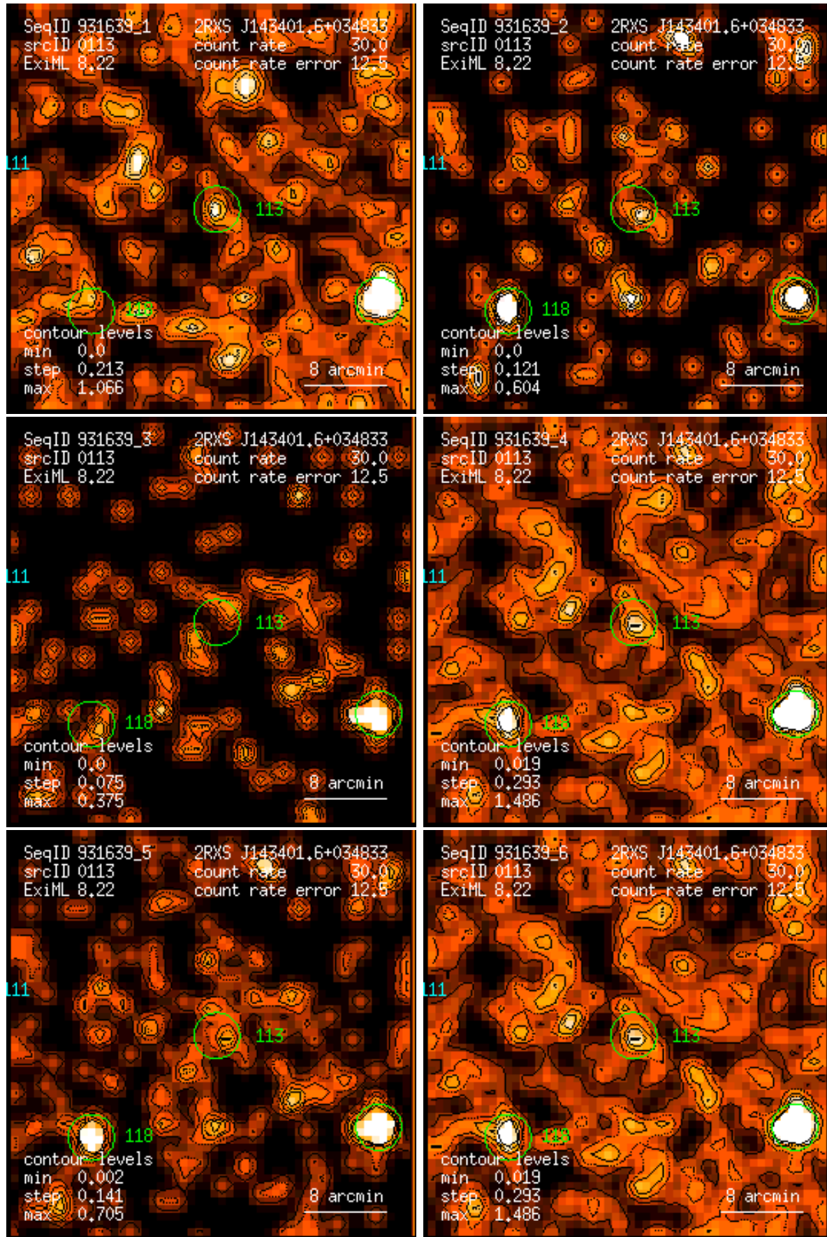
Figure 113: RASS 931639: detection 0113: band rate images, Gaussian filter: (1) PSPC channels 11 – 41, (2) 52 – 90, (3) 91 – 201, (4) 11 – 235, (5) 52 – 201, (6) 11 – 201. Broad band rates in counts/ks. Band rate contour levels in counts/ks/arcmin 2 .
