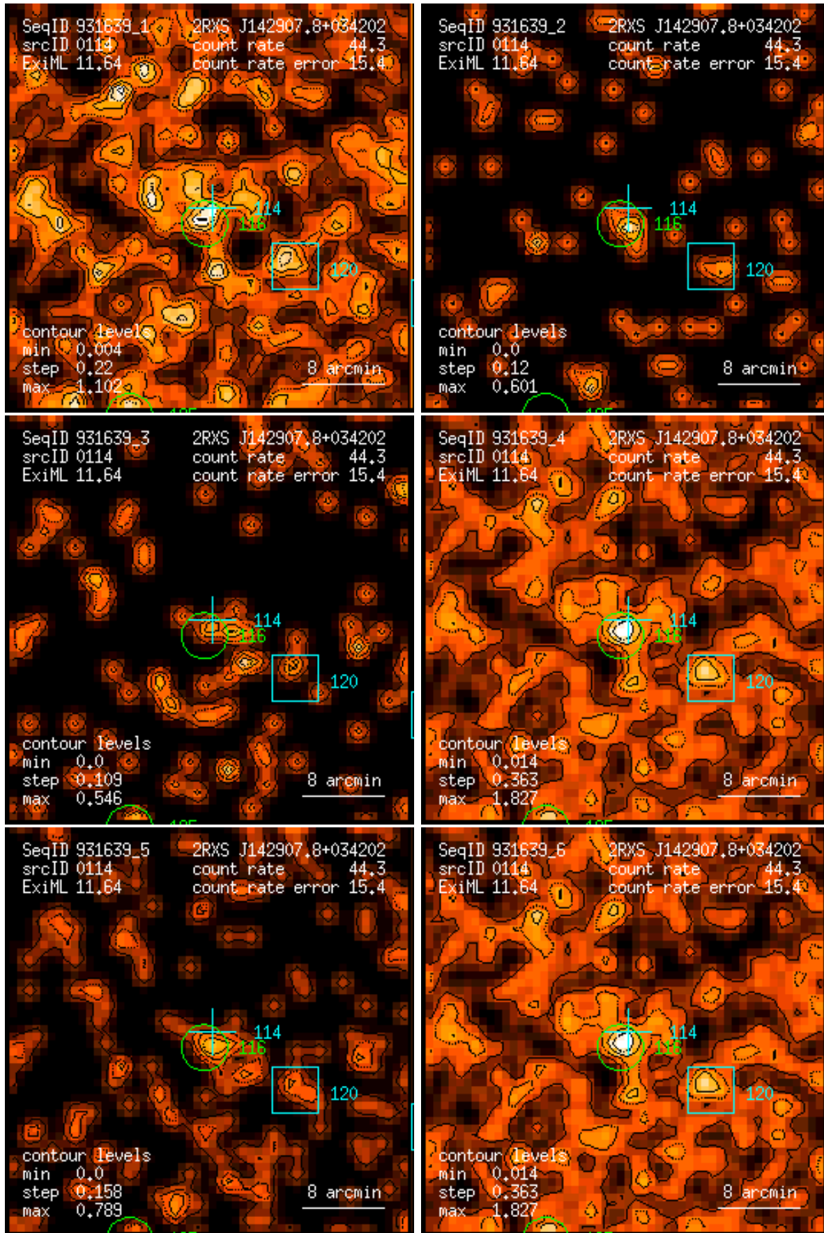
Figure 114: RASS 931639: detection 0114: band rate images, Gaussian filter: (1) PSPC channels 11 – 41, (2) 52 – 90, (3) 91 – 201, (4) 11 – 235, (5) 52 – 201, (6) 11 – 201. Broad band rates in counts/ks. Band rate contour levels in counts/ks/arcmin 2 .
