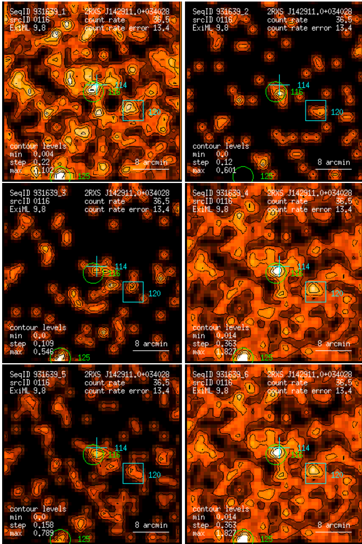
Figure 116: RASS 931639: detection 0116: band rate images, Gaussian filter: (1) PSPC channels 11 – 41, (2) 52 – 90, (3) 91 – 201, (4) 11 – 235, (5) 52 – 201, (6) 11 – 201. Broad band rates in counts/ks. Band rate contour levels in counts/ks/arcmin 2 .
