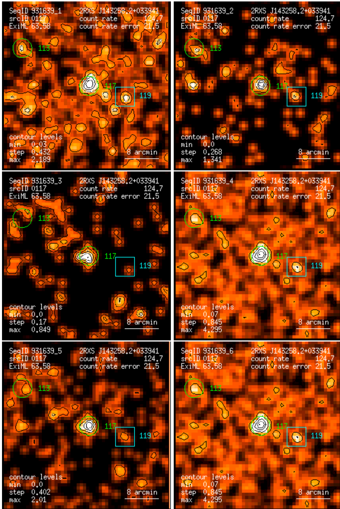
Figure 117: RASS 931639: detection 0117: band rate images, Gaussian filter: (1) PSPC channels 11 – 41, (2) 52 – 90, (3) 91 – 201, (4) 11 – 235, (5) 52 – 201, (6) 11 – 201. Broad band rates in counts/ks. Band rate contour levels in counts/ks/arcmin 2 .
