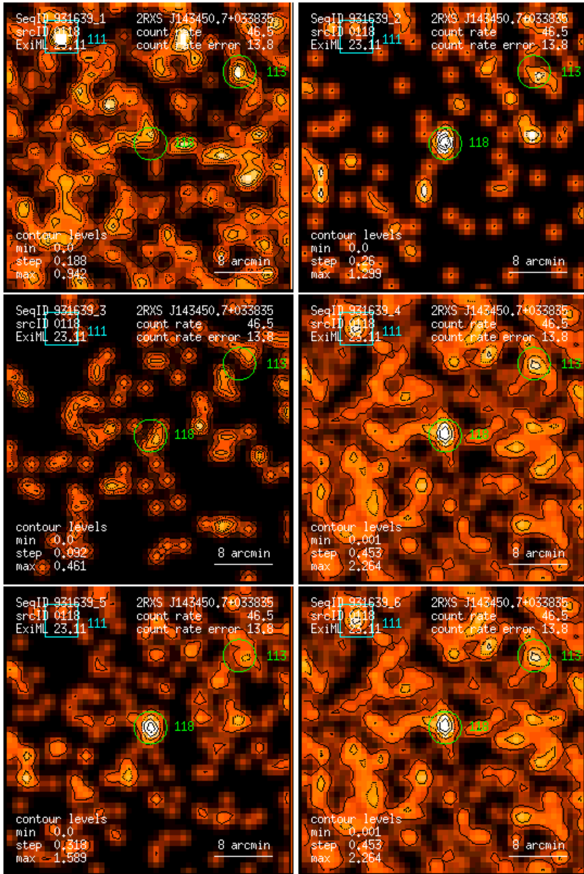
Figure 118: RASS 931639: detection 0118: band rate images, Gaussian filter: (1) PSPC channels 11 – 41, (2) 52 – 90, (3) 91 – 201, (4) 11 – 235, (5) 52 – 201, (6) 11 – 201. Broad band rates in counts/ks. Band rate contour levels in counts/ks/arcmin 2 .
