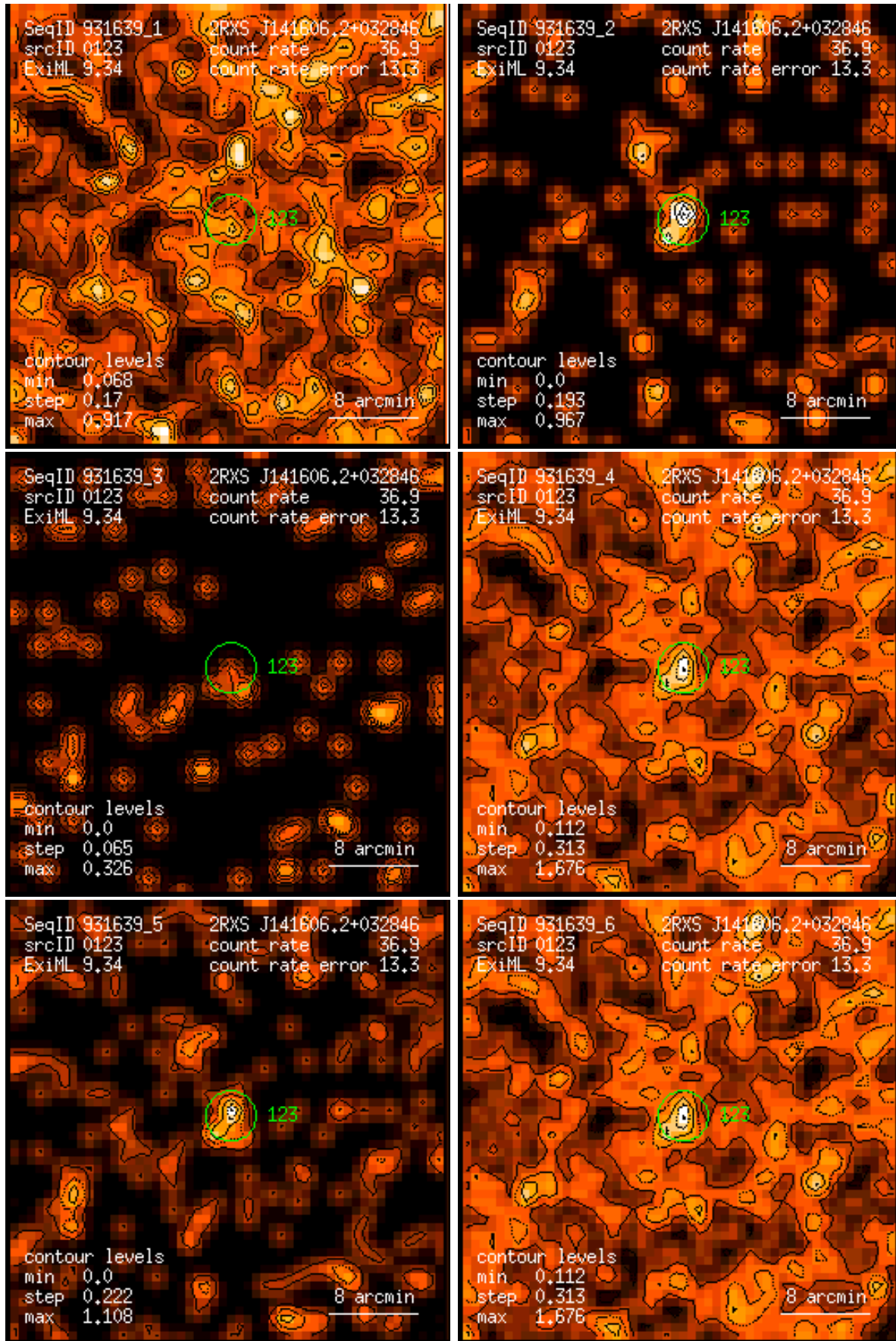
Figure 123: RASS 931639: detection 0123: band rate images, Gaussian filter: (1) PSPC channels 11 – 41, (2) 52 – 90, (3) 91 – 201, (4) 11 – 235, (5) 52 – 201, (6) 11 – 201. Broad band rates in counts/ks. Band rate contour levels in counts/ks/arcmin 2 .
