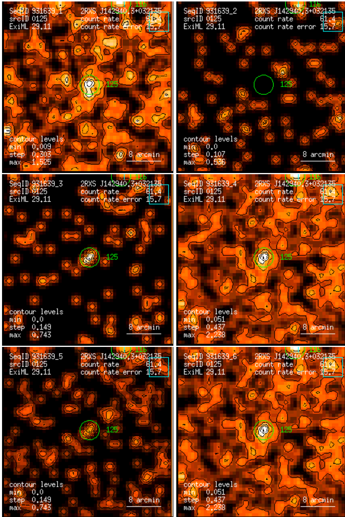
Figure 125: RASS 931639: detection 0125: band rate images, Gaussian filter: (1) PSPC channels 11 – 41, (2) 52 – 90, (3) 91 – 201, (4) 11 – 235, (5) 52 – 201, (6) 11 – 201. Broad band rates in counts/ks. Band rate contour levels in counts/ks/arcmin 2 .
