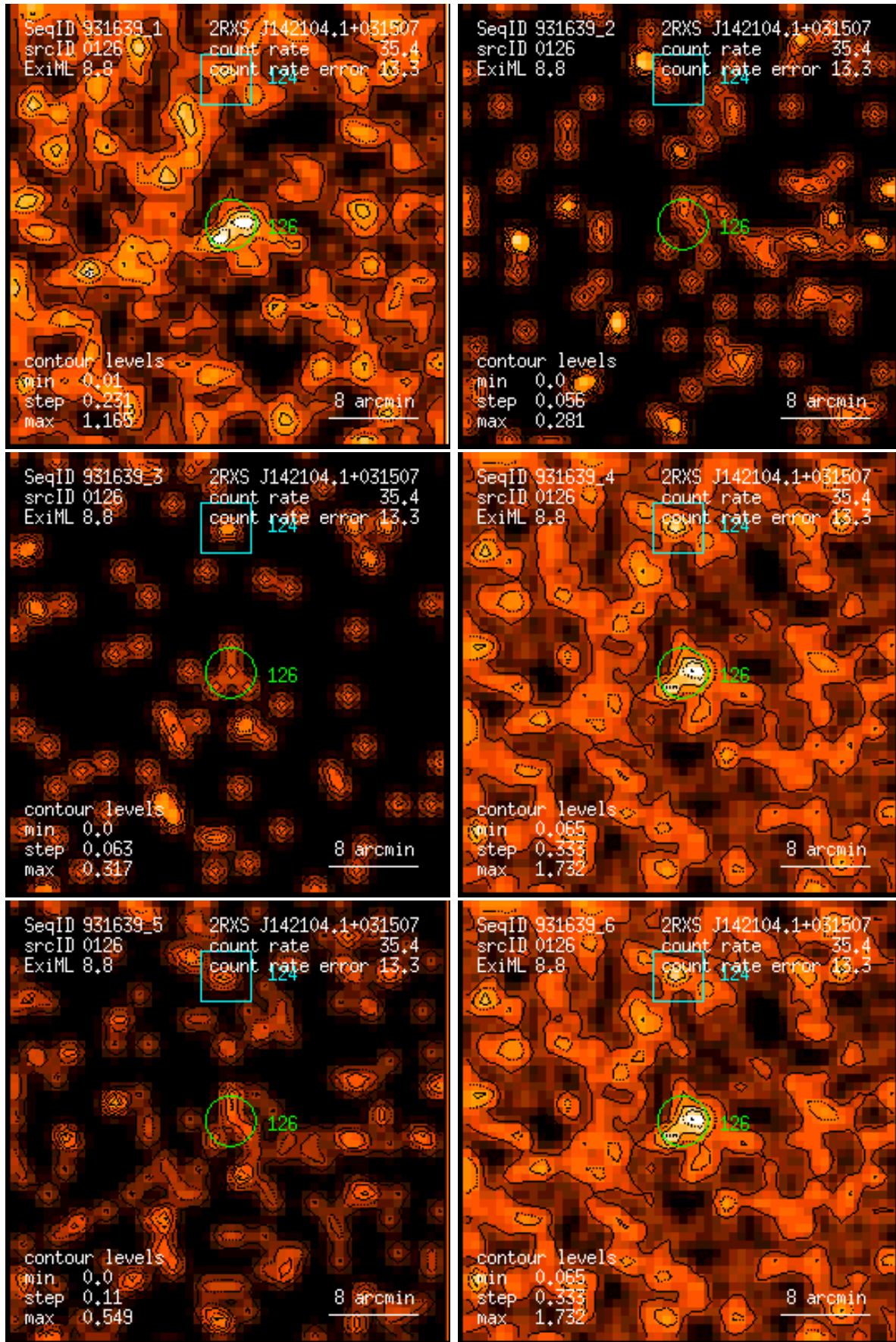
Figure 126: RASS 931639: detection 0126: band rate images, Gaussian filter: (1) PSPC channels 11 – 41, (2) 52 – 90, (3) 91 – 201, (4) 11 – 235, (5) 52 – 201, (6) 11 – 201. Broad band rates in counts/ks. Band rate contour levels in counts/ks/arcmin 2 .
