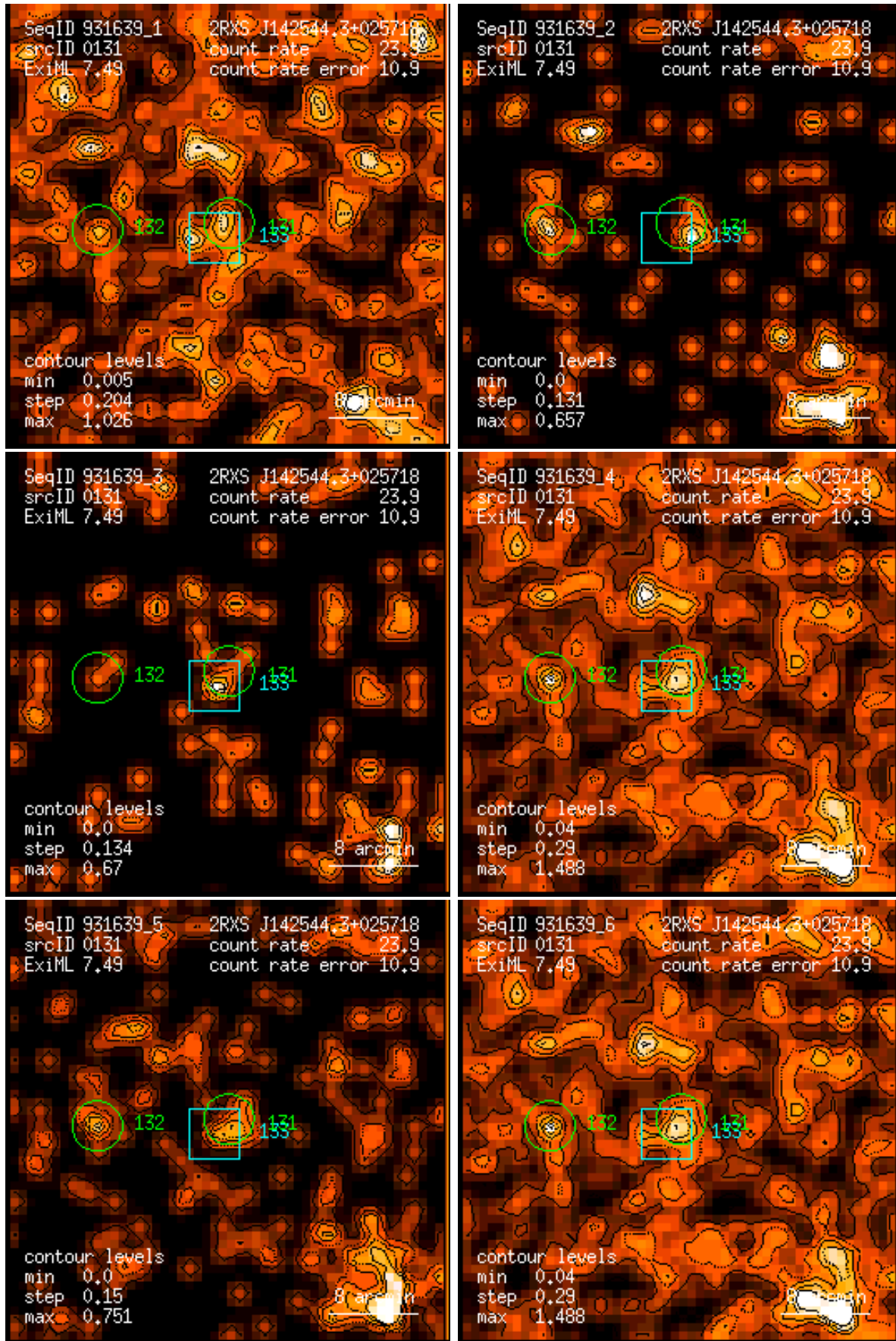
Figure 131: RASS 931639: detection 0131: band rate images, Gaussian filter: (1) PSPC channels 11 – 41, (2) 52 – 90, (3) 91 – 201, (4) 11 – 235, (5) 52 – 201, (6) 11 – 201. Broad band rates in counts/ks. Band rate contour levels in counts/ks/arcmin 2 .
