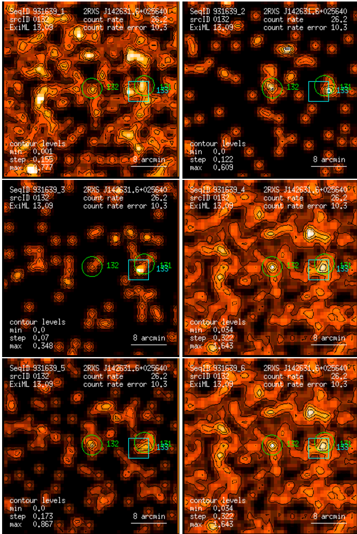
Figure 132: RASS 931639: detection 0132: band rate images, Gaussian filter: (1) PSPC channels 11 – 41, (2) 52 – 90, (3) 91 – 201, (4) 11 – 235, (5) 52 – 201, (6) 11 – 201. Broad band rates in counts/ks. Band rate contour levels in counts/ks/arcmin 2 .
