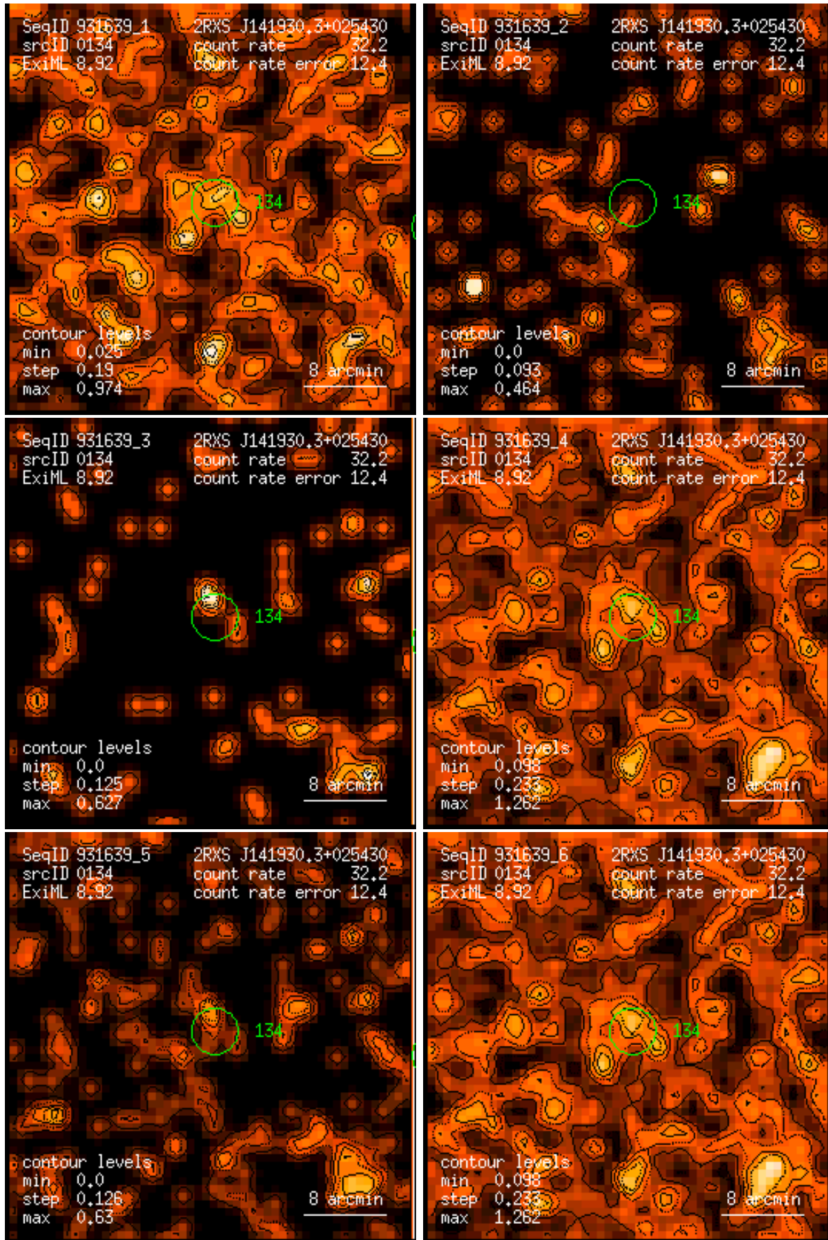
Figure 134: RASS 931639: detection 0134: band rate images, Gaussian filter: (1) PSPC channels 11 – 41, (2) 52 – 90, (3) 91 – 201, (4) 11 – 235, (5) 52 – 201, (6) 11 – 201. Broad band rates in counts/ks. Band rate contour levels in counts/ks/arcmin 2 .
