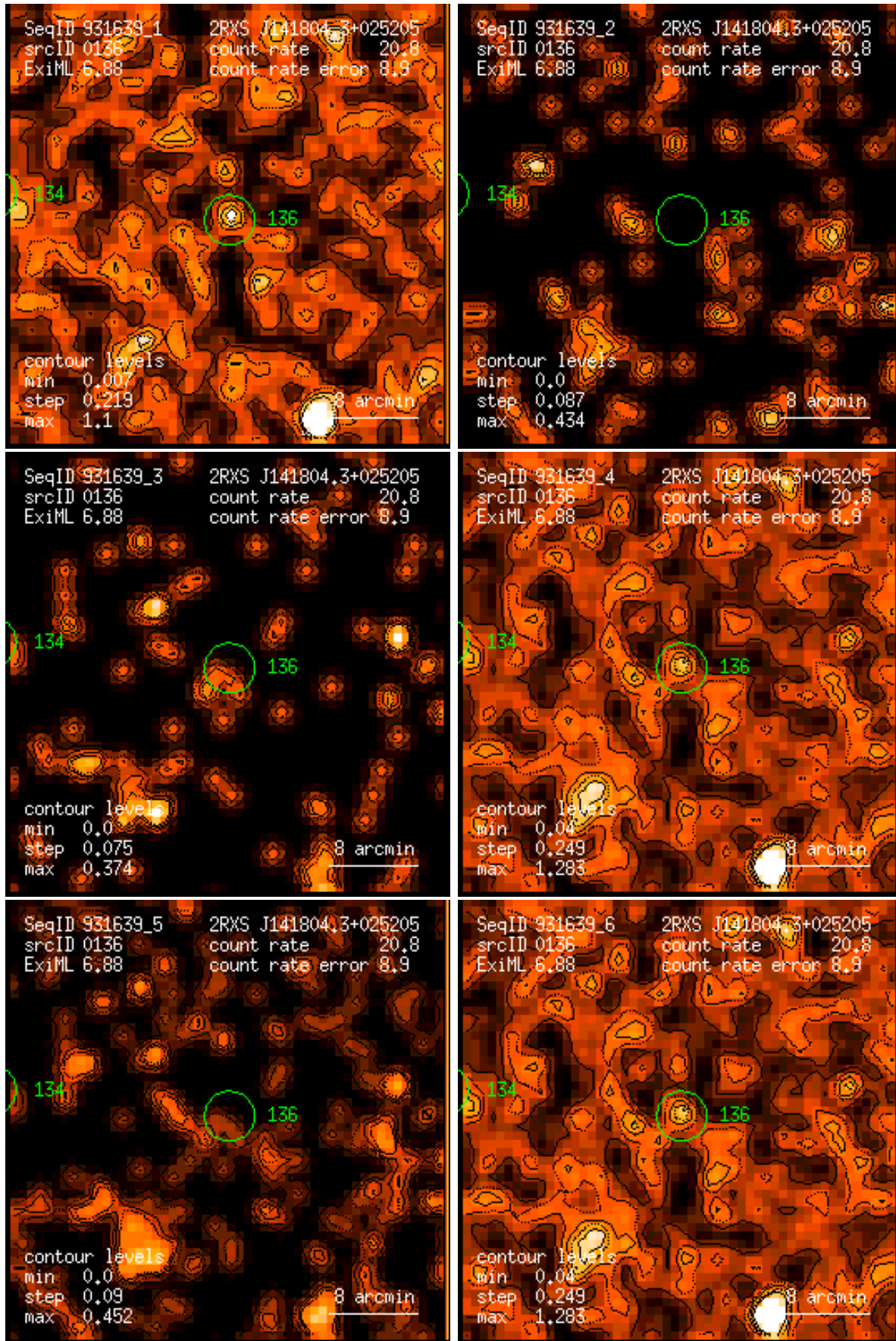
Figure 136: RASS 931639: detection 0136: band rate images, Gaussian filter: (1) PSPC channels 11 – 41, (2) 52 – 90, (3) 91 – 201, (4) 11 – 235, (5) 52 – 201, (6) 11 – 201. Broad band rates in counts/ks. Band rate contour levels in counts/ks/arcmin 2 .
