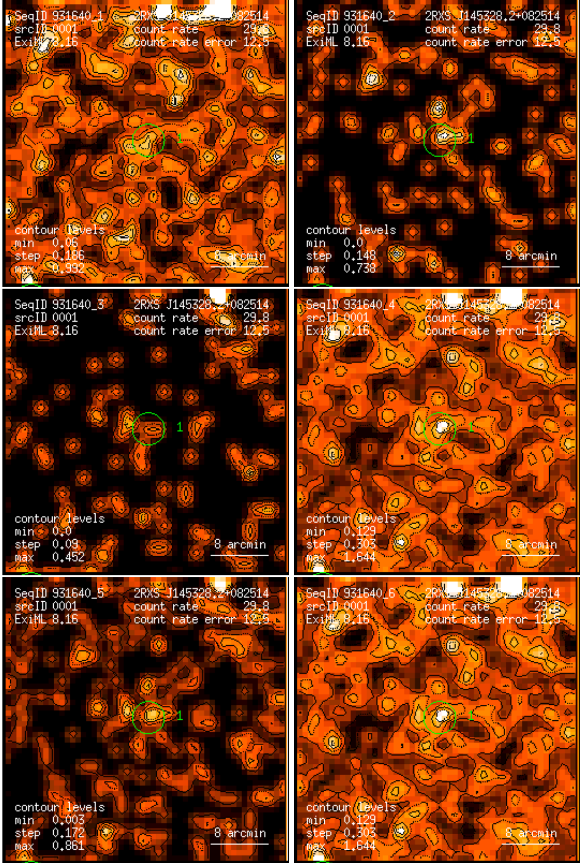
Figure 1: RASS 931640: detection 0001: band rate images, Gaussian filter: (1) PSPC channels 11 – 41, (2) 52 – 90, (3) 91 – 201, (4) 11 – 235, (5) 52 – 201, (6) 11 – 201. Broad band rates in counts/ks. Band rate contour levels in counts/ks/arcmin 2 .
