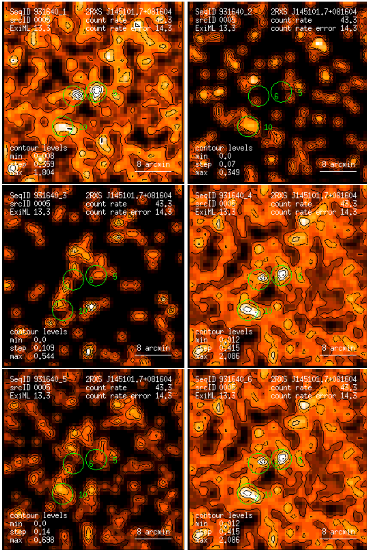
Figure 5: RASS 931640: detection 0005: band rate images, Gaussian filter: (1) PSPC channels 11 – 41, (2) 52 – 90, (3) 91 – 201, (4) 11 – 235, (5) 52 – 201, (6) 11 – 201. Broad band rates in counts/ks. Band rate contour levels in counts/ks/arcmin 2 .
